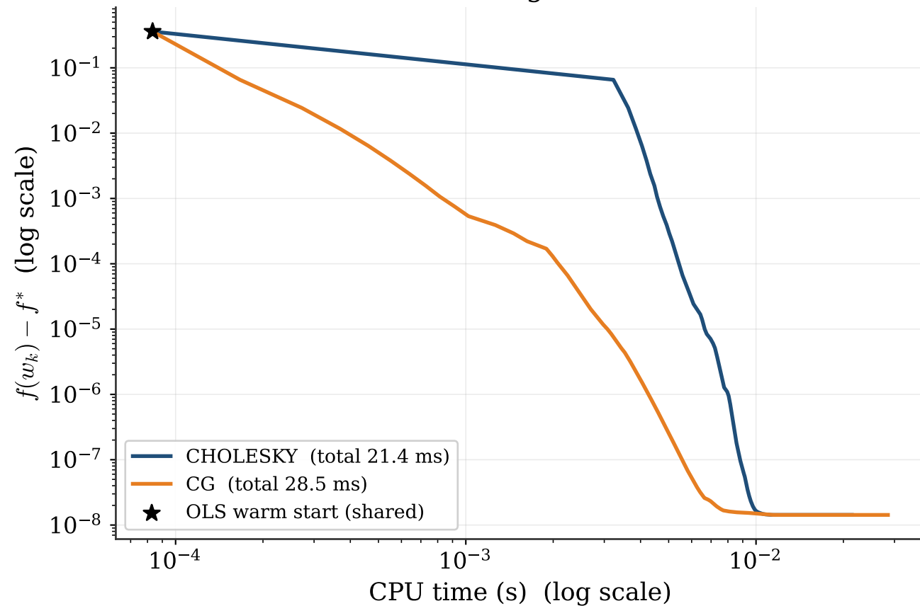
IRLS solver: convergence vs CPU time
