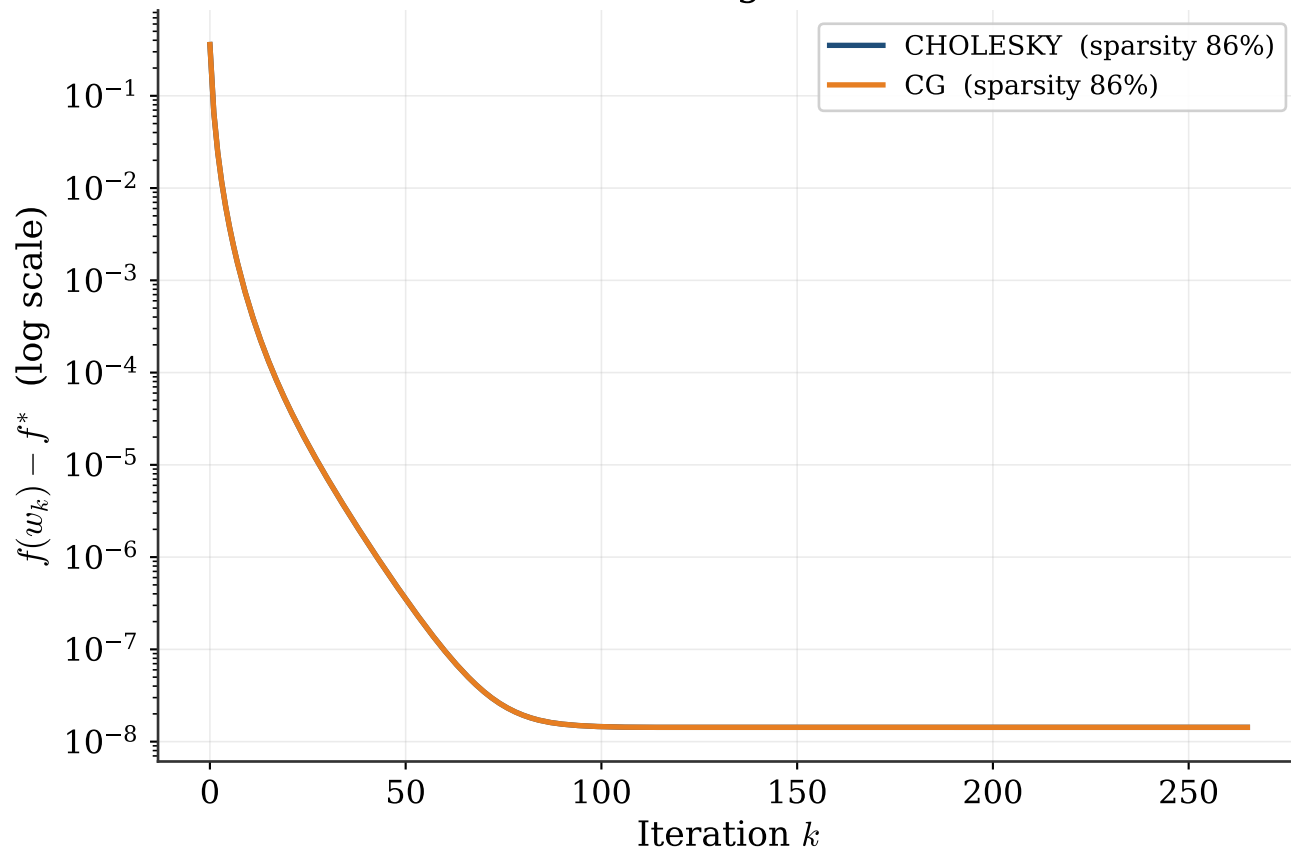
IRLS solver: convergence vs iterations
