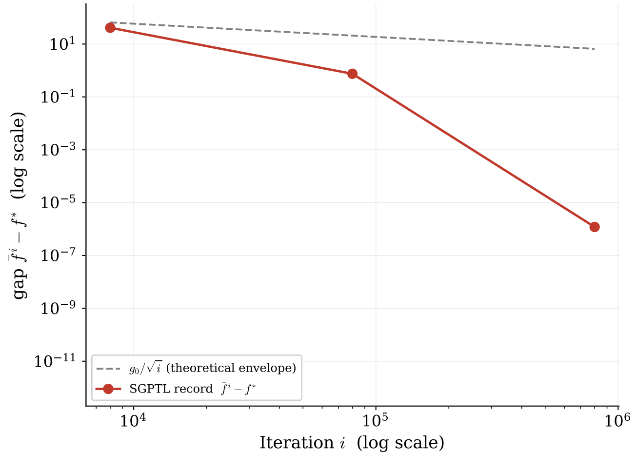
california cold start ( H = 200 , \lambda = 0.1 , i_{\max} = 800,000 )
