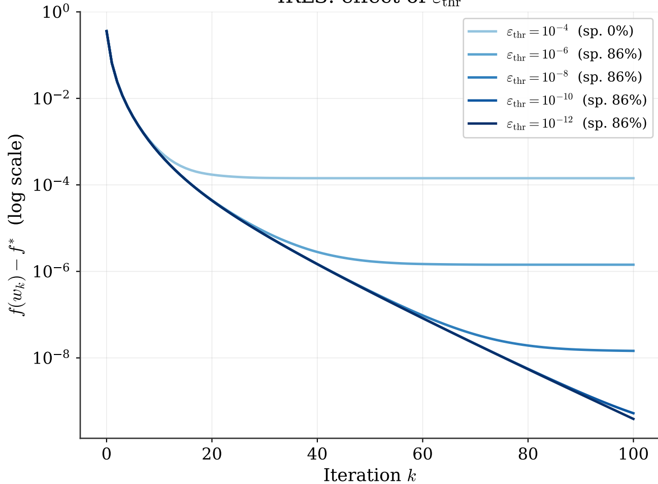
IRLS: effect of \varepsilon_{\text{thr}}
