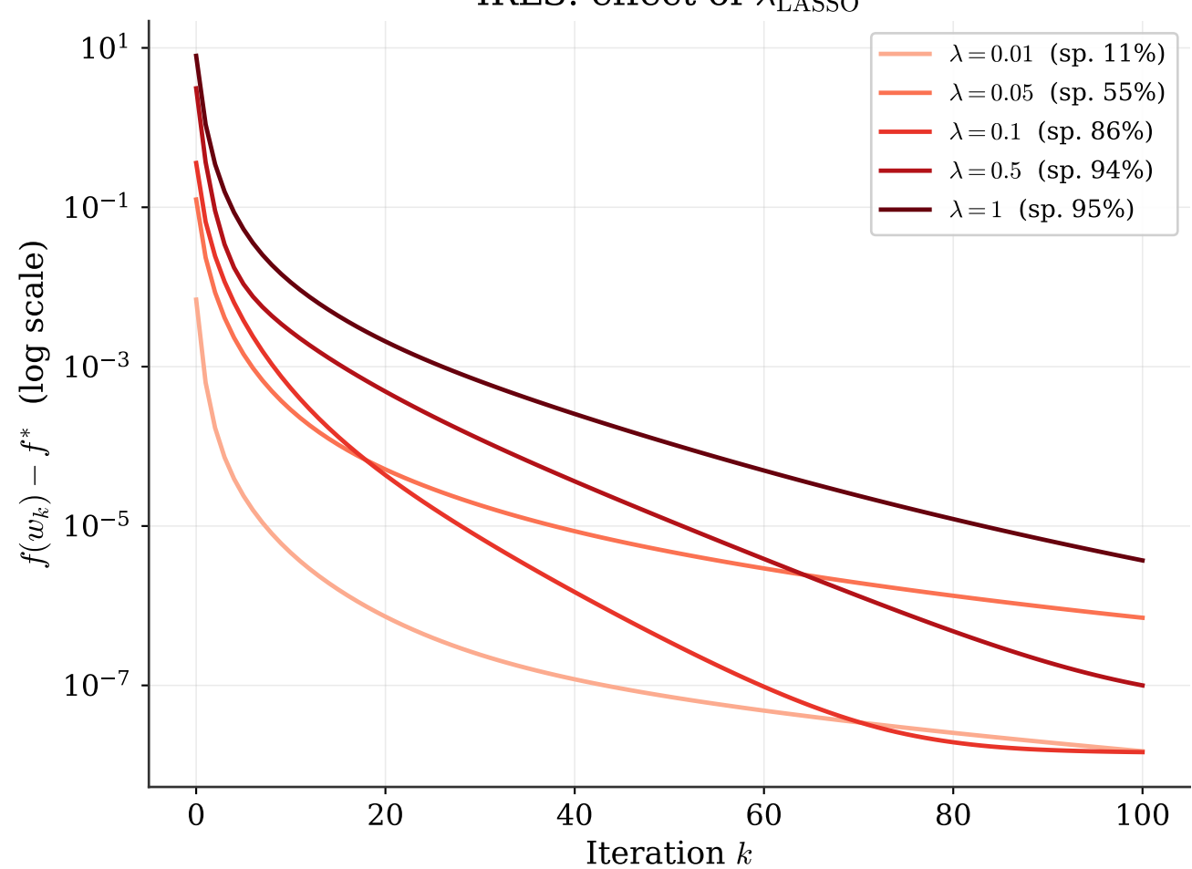
IRLS: effect of \lambda_{\text{LASSO}}
