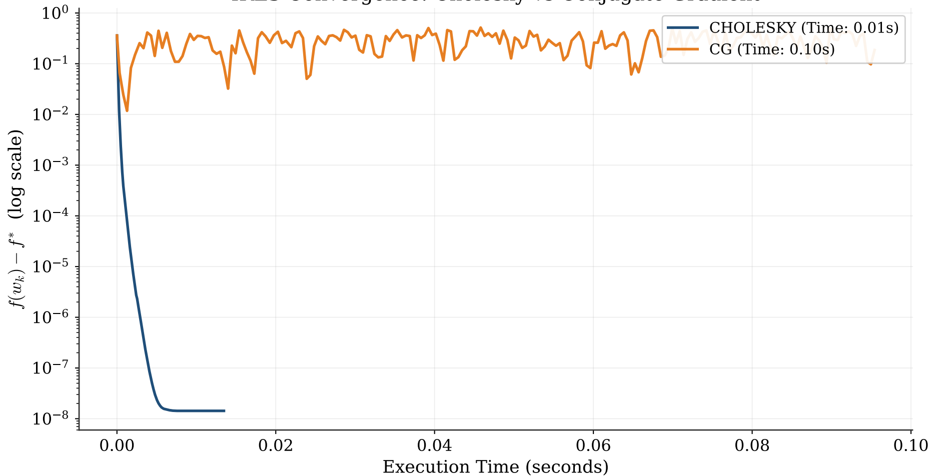
IRLS Convergence: Cholesky vs Conjugate Gradient
