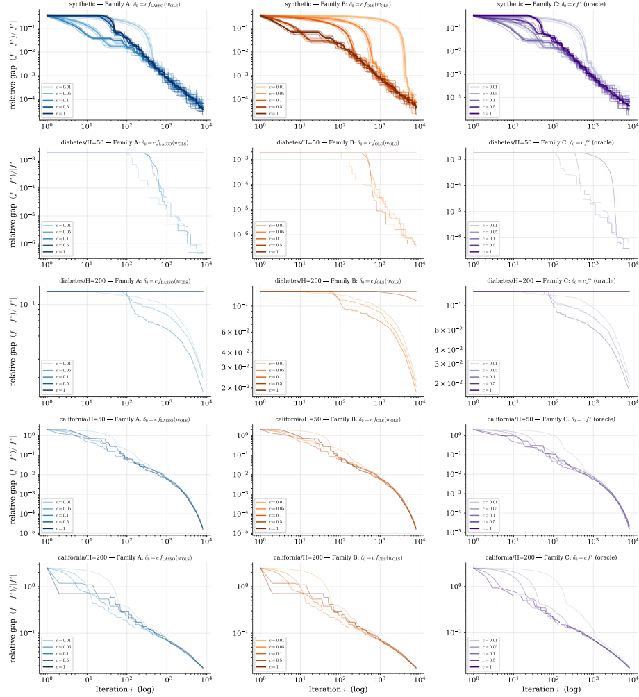
Figure A.1: Sensitivity of the final record relative gap (f - f^*)/|f^*| to \delta_0 , three families across five instances (rows): synthetic (5 seeds, per-seed thin traces and aggregate-mean thick), diabetes H = 50 (warm), diabetes H = 200 (warm), california H = 50 (cold), california H = 200 (cold). All runs use \lambda_{\text{LASSO}} = 0.1 , \rho = 0.7 , \gamma_{\min} = 0.05 , i_{\max} = 8000 . Family A: \delta_0 = c f(\mathbf{w}_0) (default). Family B: \delta_0 = c \frac{1}{2} \|\mathbf{X}\mathbf{w}_0 - \mathbf{y}\|^2 . Family C: \delta_0 = c f^* (oracle, inadmissible). The Family A/Family C ratio falls in [0.5, 2.0] in every regime where SGPTL admits progress.
