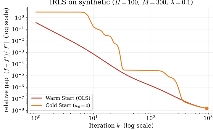
Figure B.1: IRLS warm (OLS) vs cold ( \mathbf{w}_0 = \mathbf{0} ) start on the synthetic instance ( H = 100 , M = 300 , \lambda_{\text{LASSO}} = 0.1 , k_{\text{max}} = 2000 , \varepsilon_{\text{thr}} = 10^{-8} ), log-log axes, relative gap (f - f^*)/|f^*| . Both starts converge to the \varepsilon_{\text{thr}} floor ( (f - f^*)/|f^*| \approx 1.6 \cdot 10^{-8} ) at iteration 940 (warm) and 922 (cold); the warm curve sits below the cold one throughout the descent, consistent with the multiplicative role of \|\mathbf{w}_0 - \mathbf{w}^*\| in the bound of Section 2.5.
