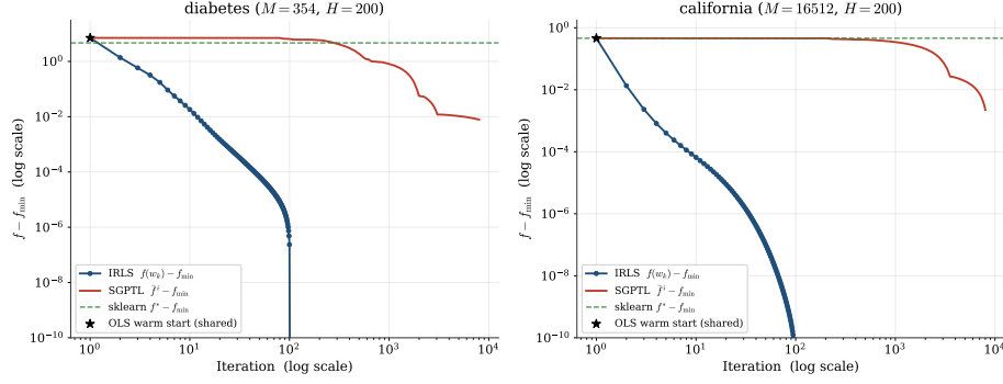
Figure 5.9: Convergence on the two real datasets, log-log axes, plotting f - f_{\min} with f_{\min} the lowest objective any of \{\text{IRLS}, \text{SGPTL}, \text{sklearn}\} attained on the dataset. The star marks the OLS warm start (shared by both algorithms) and the dashed green line marks sklearn's f^* - f_{\min} where the sklearn run finished (skipped on California, see Table 5.4). Both IRLS and SGPTL drop below the sklearn reference within their respective budgets; IRLS reaches the 10^{-10} display floor within \sim 100 iterations, SGPTL converges sublinearly to a gap of \sim 10^{-2} (diabetes) or \sim 3 \cdot 10^{-3} (California) at i_{\max} = 8000 . The panels confirm that the synthetic-instance picture (Section 5.2) carries through to the real datasets: SGPTL converges, just much more slowly than IRLS.
