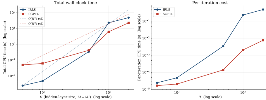
Figure 5.7: Scaling of wall-clock time with H at M = 5H . Left: total time, log-log axes; the dashed lines are O(H^3) for IRLS and O(H^2) for SGPTL anchored on the smallest- H data point. Right: per-iteration cost. SGPTL tracks the O(H^2) slope; IRLS’ total cost departs from the cubic prediction at H \geq 1000 , where the Cholesky factor outgrows the L2 cache.
