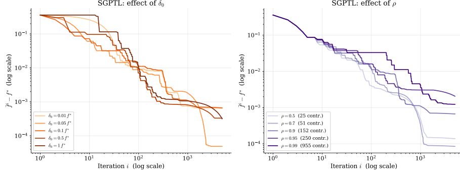
Figure 5.6: SGPTL sensitivity ( H = 100 , M = 400 , OLS warm start, 5000 iterations). Left: effect of \delta_0 as a fraction of f^* at \rho = 0.9 — final gaps cluster in [5 \cdot 10^{-5}, 7 \cdot 10^{-4}] , the algorithm is robust to \delta_0 . Right: effect of \rho at \delta_0 = 0.1 f^* ; aggressive contraction ( \rho = 0.7 ) reaches 8.5 \cdot 10^{-5} , slow contraction ( \rho = 0.99 ) plateaus at 1.2 \cdot 10^{-3} . The contraction count is reported in each legend.
