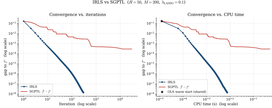
Figure 5.8: IRLS versus SGPTL on the moderate problem ( H = 50, M = 200, \lambda_{\text{LASSO}} = 0.1 ). Both panels use log–log axes: linear scaling would crush IRLS’ \sim 100 iterations against the axis next to SGPTL’s 30000. Left: optimality gap versus iteration. Right: gap versus CPU time. SGPTL falls below 10^{-2} in 22 iterations and 10^{-3} in 564, then enters the sublinear regime; IRLS reaches 10^{-8} within \sim 10 ms.
