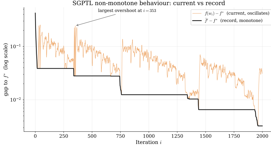
Figure 5.4: SGPTL on the convergence instance, first 2000 iterations, semilog y axis. The current gap f(\mathbf{w}_i) - f^* (orange) spikes well above the record gap \hat{f}^i - f^* (black) at several points throughout the run, while the record is monotone non-increasing by construction. The largest overshoot is annotated. This is the practical reason why the algorithm returns \mathbf{w}_{\text{best}} rather than the last iterate.
