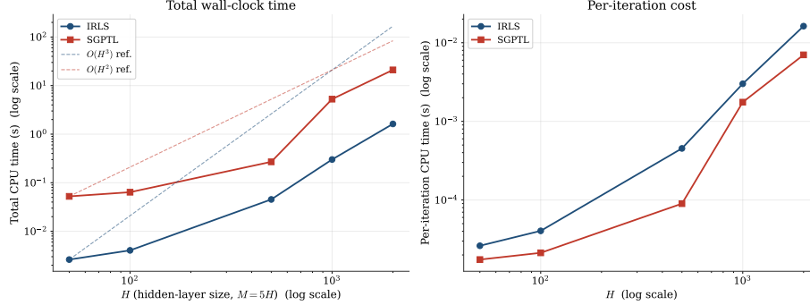
Figure 5.8: Scaling of wall-clock time with H at M = 5H . Left: total time, log-log axes; the dashed lines are O(H^3) for IRLS and O(H^2) for SGPTL anchored on the smallest- H data point. Right: per-iteration cost. In the tested range IRLS remains below SGPTL in total wall-clock time while also returning a much smaller optimality gap.
