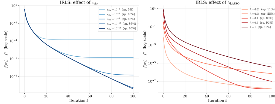
Figure 5.5: IRLS sensitivity. Left: effect of \epsilon_{\text{thr}} on convergence and sparsity at \lambda_{\text{LASSO}} = 0.1 . Right: effect of \lambda_{\text{LASSO}} at \epsilon_{\text{thr}} = 10^{-8} .
