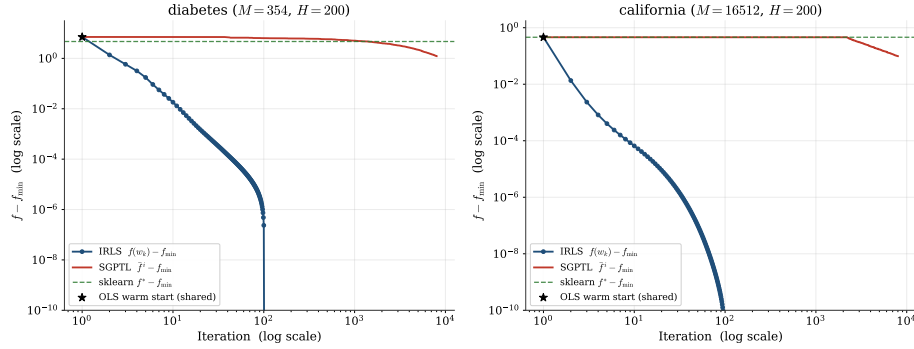
Figure 5.10: Convergence on the two real datasets, log-log axes, plotting f - f_{\min} with f_{\min} the lowest objective any of {IRLS, SGPTL, sklearn} attained on the dataset. The star marks the OLS warm start (shared by both algorithms) and the dashed green line marks sklearn's stopped value minus f_{\min} where the sklearn run finished (skipped on California, see Table 5.5). On diabetes both IRLS and SGPTL drop below the stopped sklearn objective; on California sklearn is skipped and f_{\min} is set by IRLS. IRLS reaches the display floor within \sim 100 iterations, while SGPTL converges sublinearly and remains visibly above the IRLS baseline at i_{\max} = 8000 . The panels confirm that the synthetic-instance picture (Section 5.2) carries through to the real datasets: SGPTL converges, just much more slowly than IRLS.
