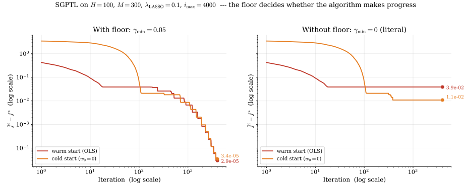
Figure 5.1: SGPTL record gap on H = 100 , M = 300 , \lambda_{\text{LASSO}} = 0.1 , i_{\max} = 4000 , log-log axes, shared y -scale. Left panel: production configuration, deflection floor \gamma_{\min} = 0.05 active. Right panel: literal projection of the greedy minimiser onto [0, 1] , i.e. \gamma_{\min} = 0 . Each panel overlays the warm and cold starts; the marker on the right end of each trace annotates the final record gap. Without the floor the iterate freezes within the first hundred iterations and the gap plateaus around 10^{-2} on both starts ( 3.9 \cdot 10^{-2} warm, 1.1 \cdot 10^{-2} cold). With \gamma_{\min} = 0.05 the clip \beta_i = \min(\beta, \gamma_i) keeps the Polyak step bounded away from zero and the gap descends three orders of magnitude further inside the same budget ( 3.0 \cdot 10^{-5} warm, 3.4 \cdot 10^{-5} cold). The deflection floor decides whether the algorithm makes progress; the choice of starting point is secondary.
