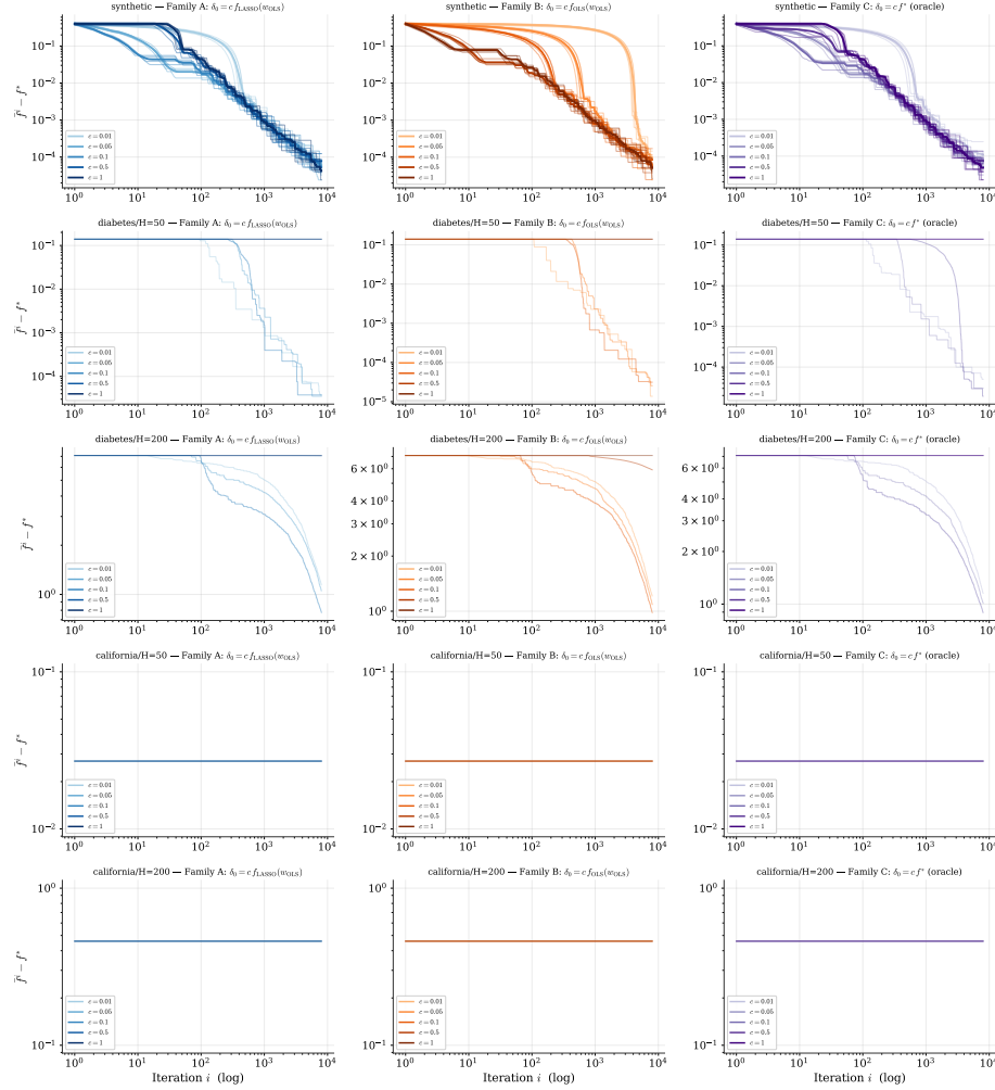
Figure 5.8: Sensitivity of the final record gap to the choice of \delta_0 , three families across five instances (rows, top to bottom): synthetic LASSO ( H = 100 , M = 300 , 5 seeds with per-seed thin traces and aggregate-mean thick), diabetes H = 50 , diabetes H = 200 , california H = 50 , california H = 200 . All runs use \rho = 0.7 , \gamma_{\min} = 0.05 , i_{\max} = 8000 . Family A: \delta_0 = c f_{\text{LASSO}}(\mathbf{w}_{\text{OLS}}) (default, admissible). Family B: \delta_0 = c \frac{1}{2} \|\mathbf{X}\mathbf{w}_{\text{OLS}} - \mathbf{y}\|^2 (admissible). Family C: \delta_0 = c f^* (diagnostic oracle, not admissible). In the working regime (top three rows where SGPTL admits progress) Families A and C agree within a factor of 2. In the stall regime (both california rows, all c ; diabetes H = 50 at c \geq 0.5 ) the three families collapse to a common plateau and the comparison is uninformative about \delta_0 but delimits SGPTL’s applicability on the column-normalised ELM transformation.
