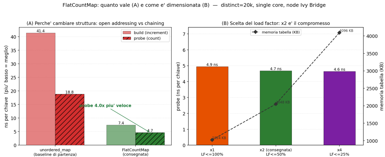
Figure 4: (A) FlatCountMap vs unordered_map: probe 4x. (B) load factor: x2 e' il compromesso.
