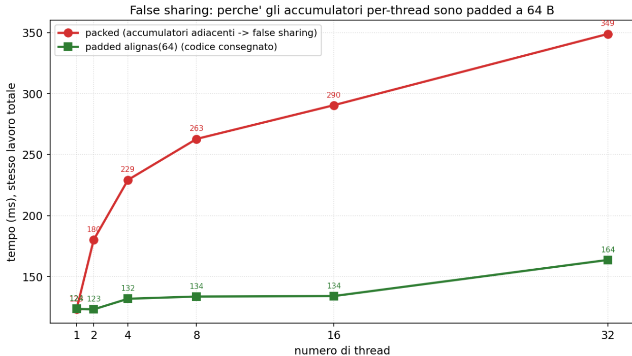
Figure 7: False sharing: accumulatori adiacenti (packed) vs padded a 64 B, stesso lavoro totale.
