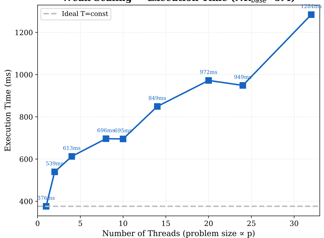
Weak Scaling — Execution Time ( NR_{base}=5M )
