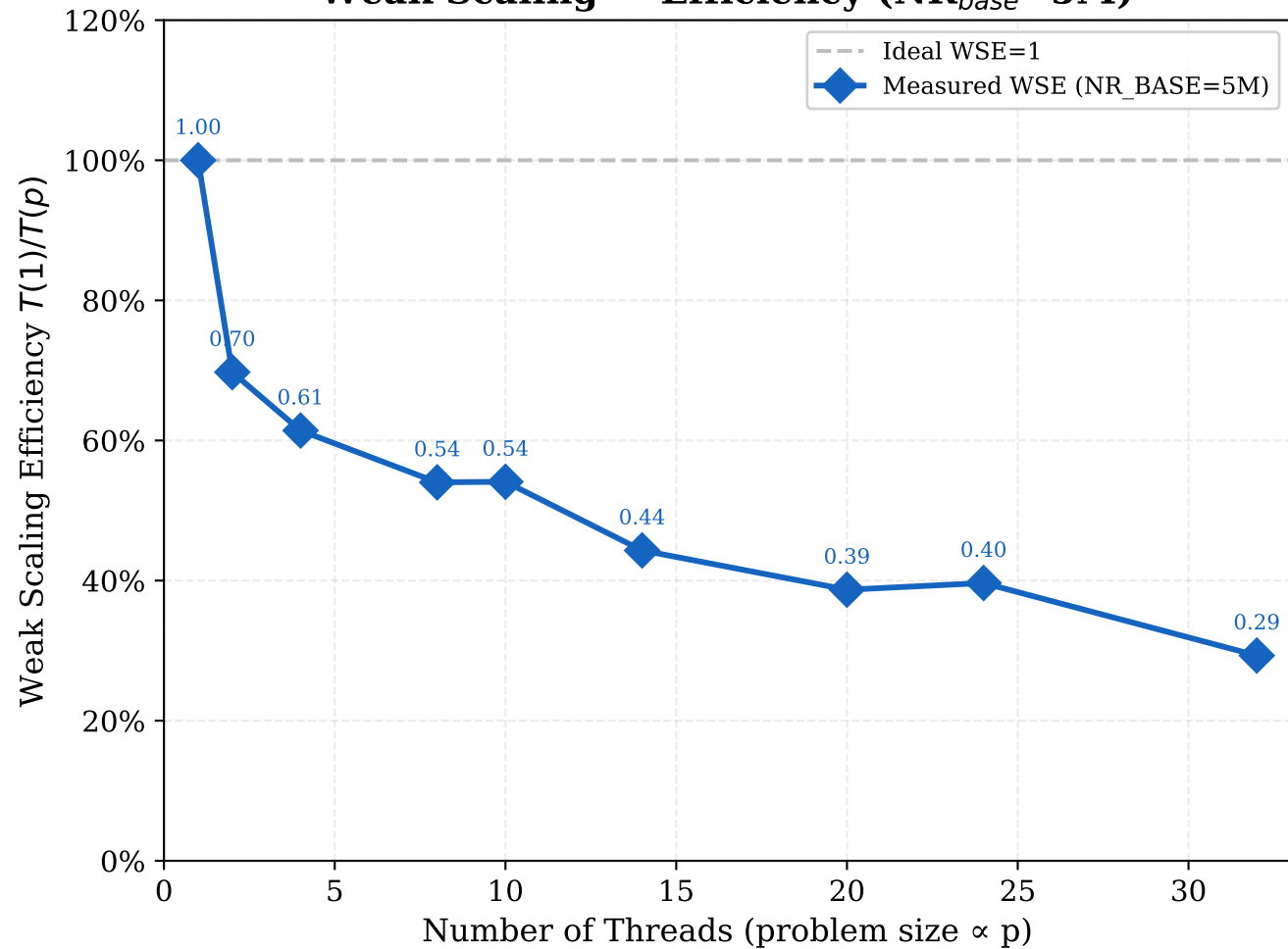
Weak Scaling — Efficiency ( NR_{base}=5M )
