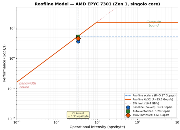
Figure 1: Roofline model. All variants sit on the bandwidth ramp ( I=0.33 ), well below compute ceilings.
