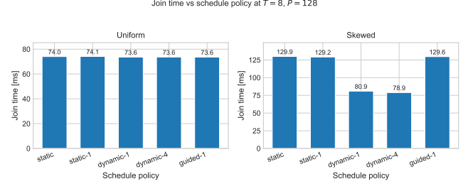
Figure 5: Join time at T = 8 across five schedule policies, uniform (left) and skewed (right). On uniform all policies fall within \sim 1\% ; on skewed the two dynamic policies are \sim 38\% faster than static/guided .
