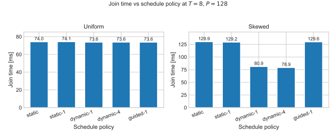
Figure 5: Join time at T=8 across five schedule policies, uniform (left) and skewed (right). On uniform all policies fall within \sim 1\% ; on skewed the two dynamic policies are \sim 38\% faster than static/guided.
