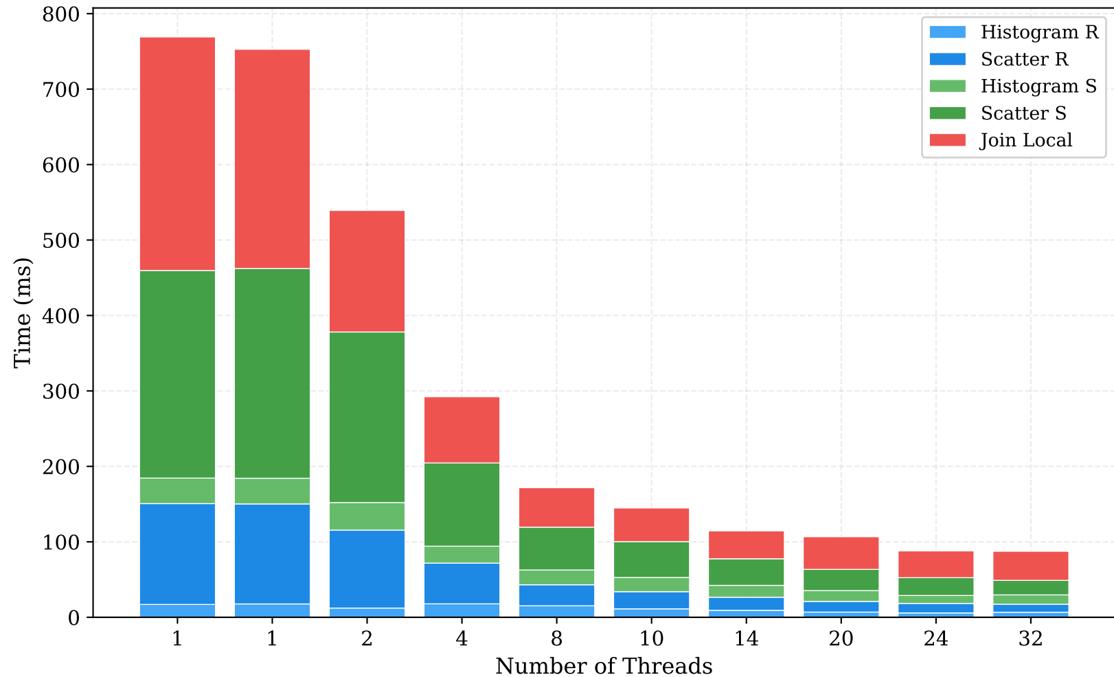
Phase Breakdown — Execution Time
