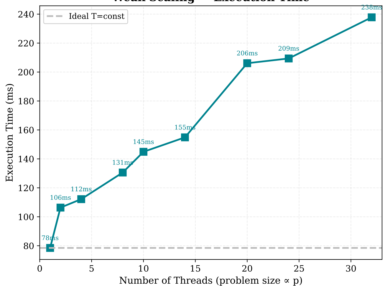
Weak Scaling — Execution Time
