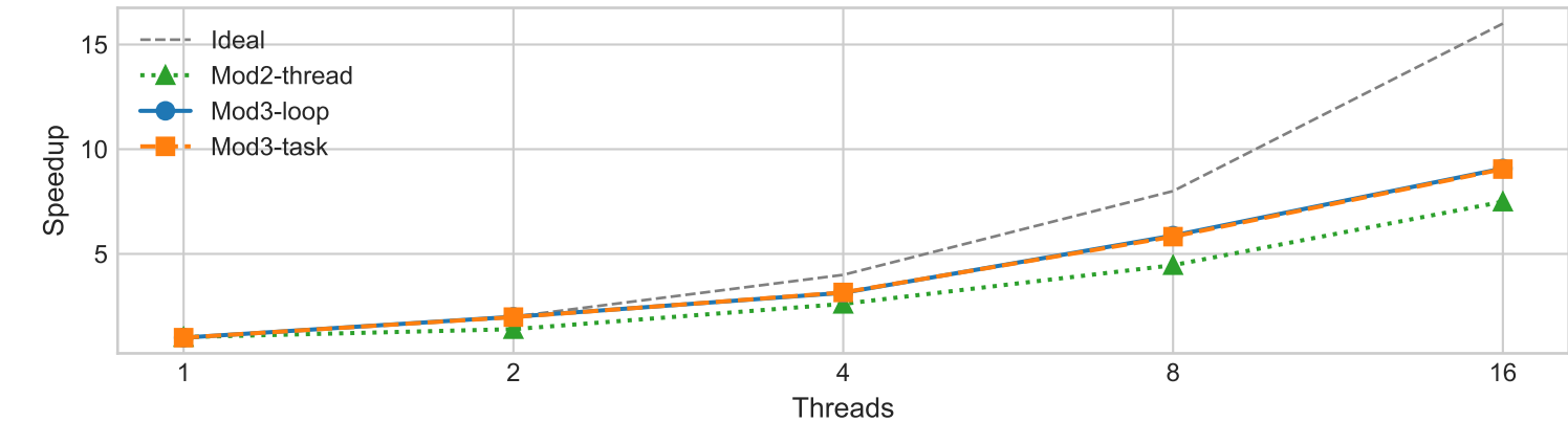
(b) Speedup
