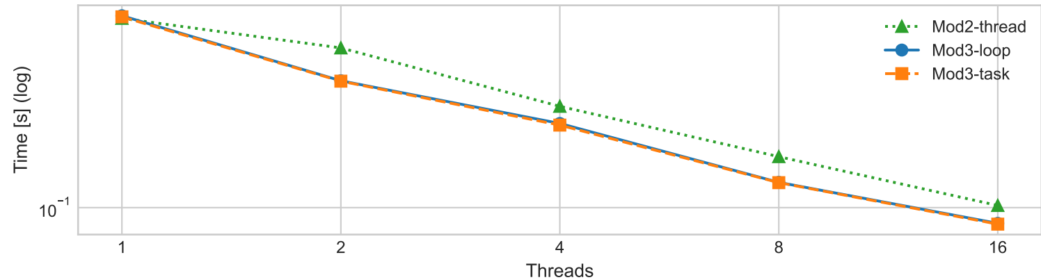
(a) Absolute time, NR=10M NS=20M uniform
