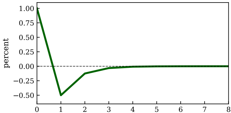
Output y_t
