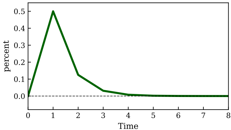
Inflation \pi_t
