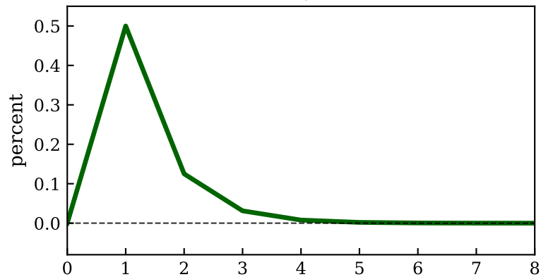
Unemployment u_t
