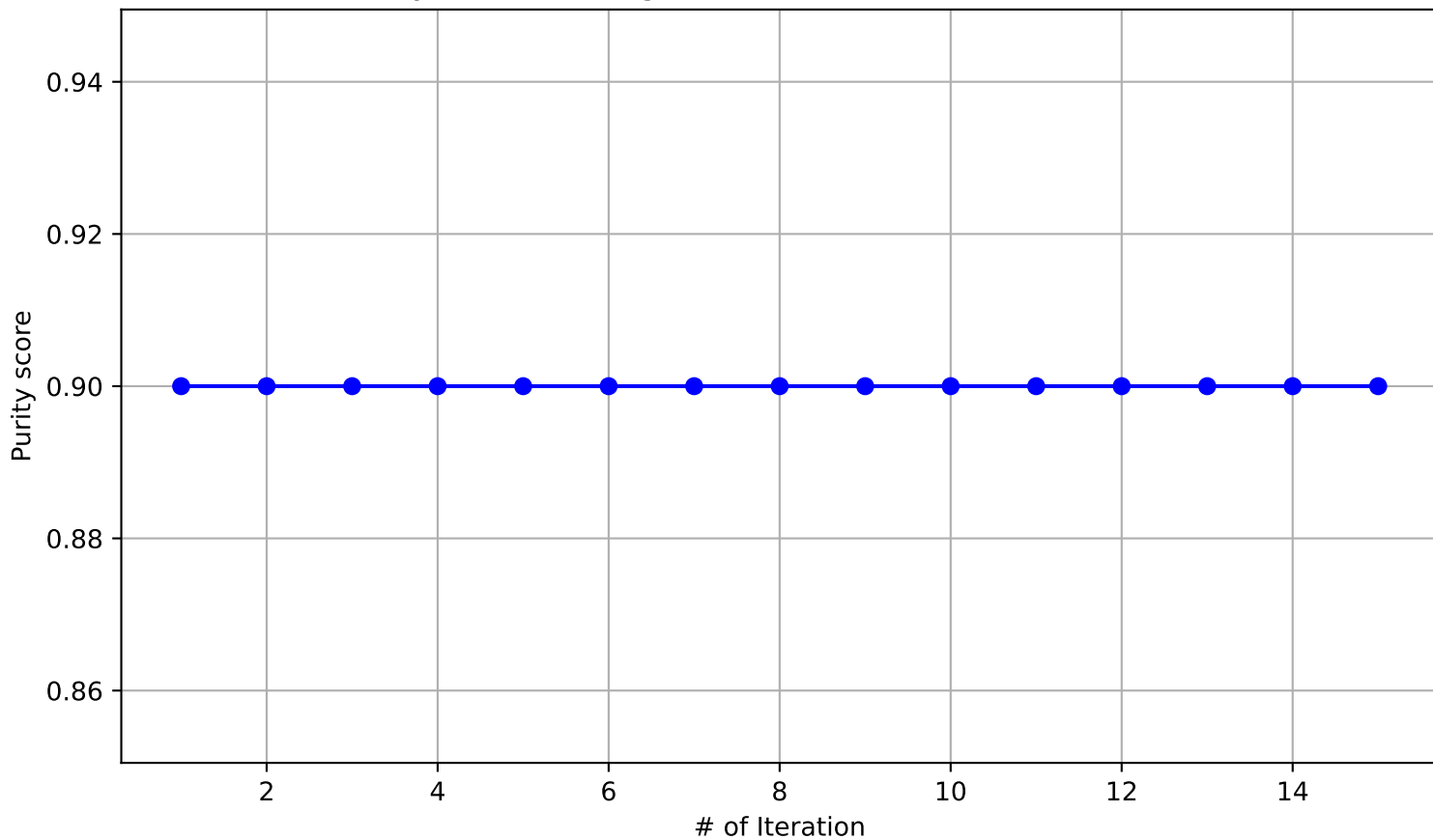
Purity score convergence of soft k-means on Iris Dataset
