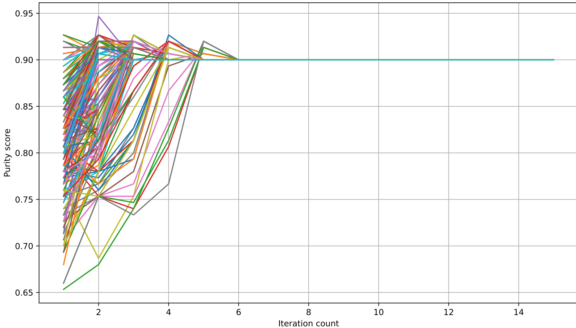
Purity score convergence across 200 random initializations
