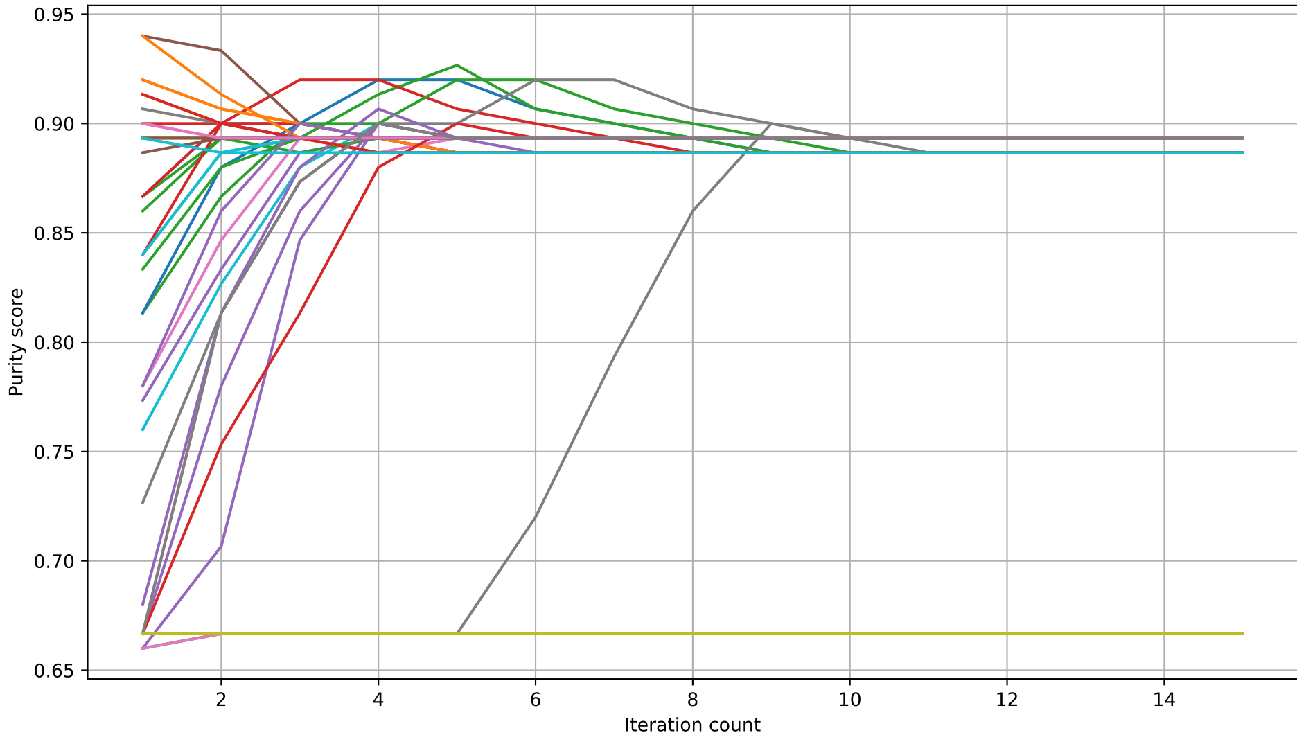
Purity score convergence across 50 random initializations
