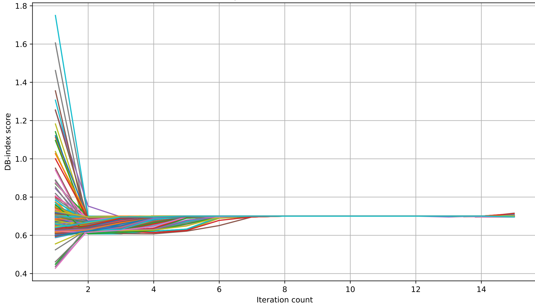
D-B score convergence across 500 random initializations
