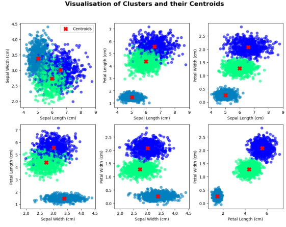
Figure 4: Gaussian Mixtures after CLL (200 steps, M = 20 )
