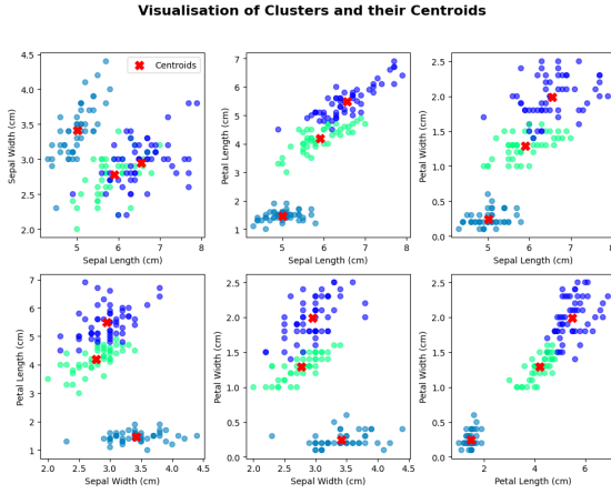
Figure 3: Gaussian Mixtures before CLL
