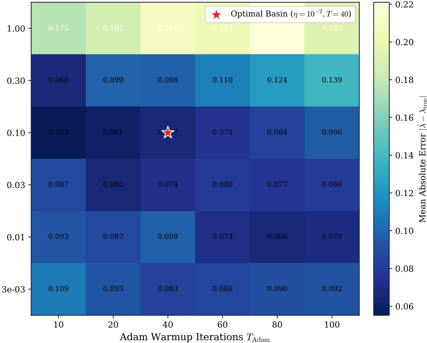
(a) Parameter Error |\hat{\lambda} - \lambda_{\text{true}}| (Lower is Better)
