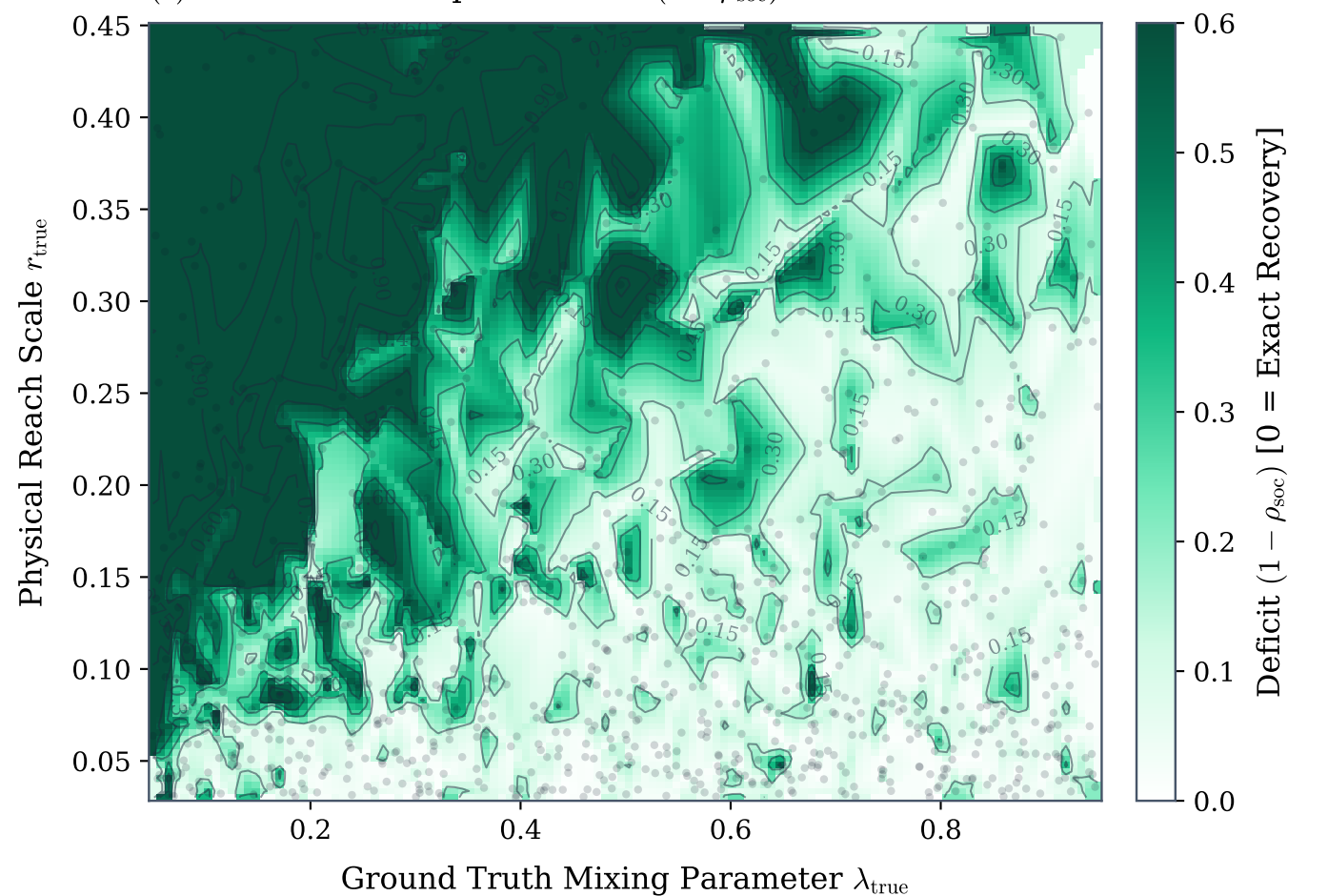
(c) Latent Metric Space Deficit (1 - \rho_{\text{soc}})
