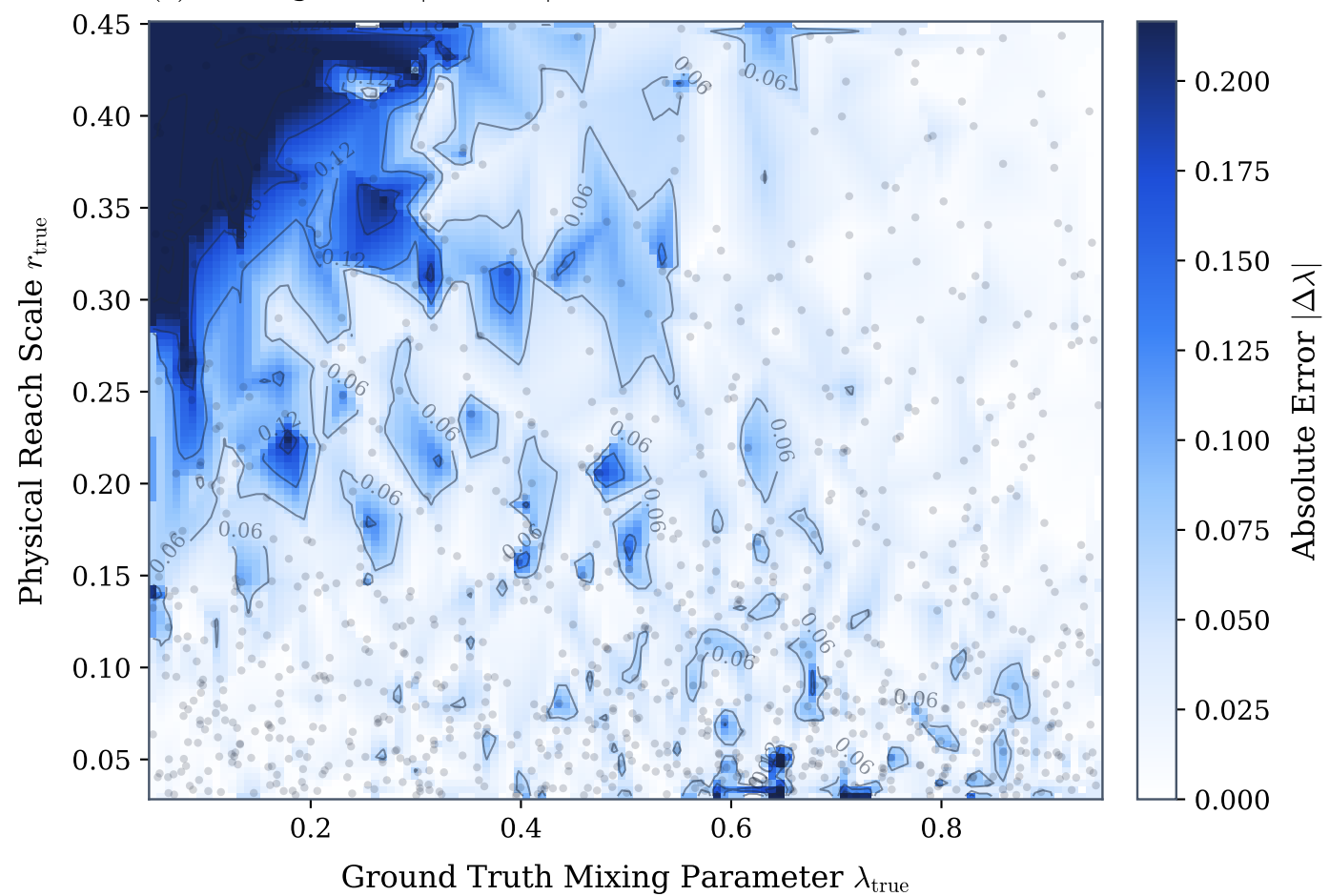
(a) Mixing Error |\hat{\lambda} - \lambda_{\text{true}}|
