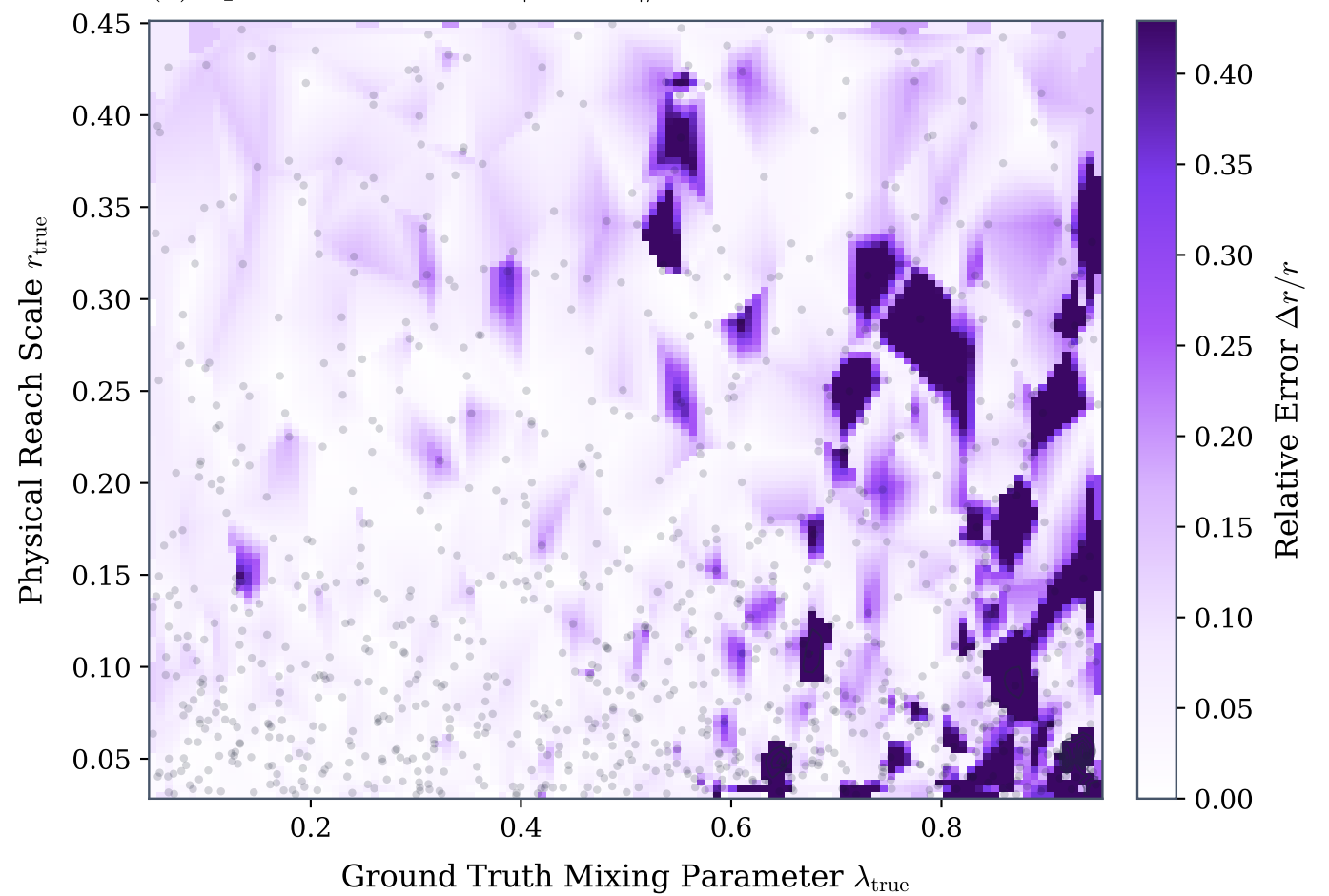
(b) Spatial Scale Error |\hat{r} - r_{\text{true}}|/r_{\text{true}}
