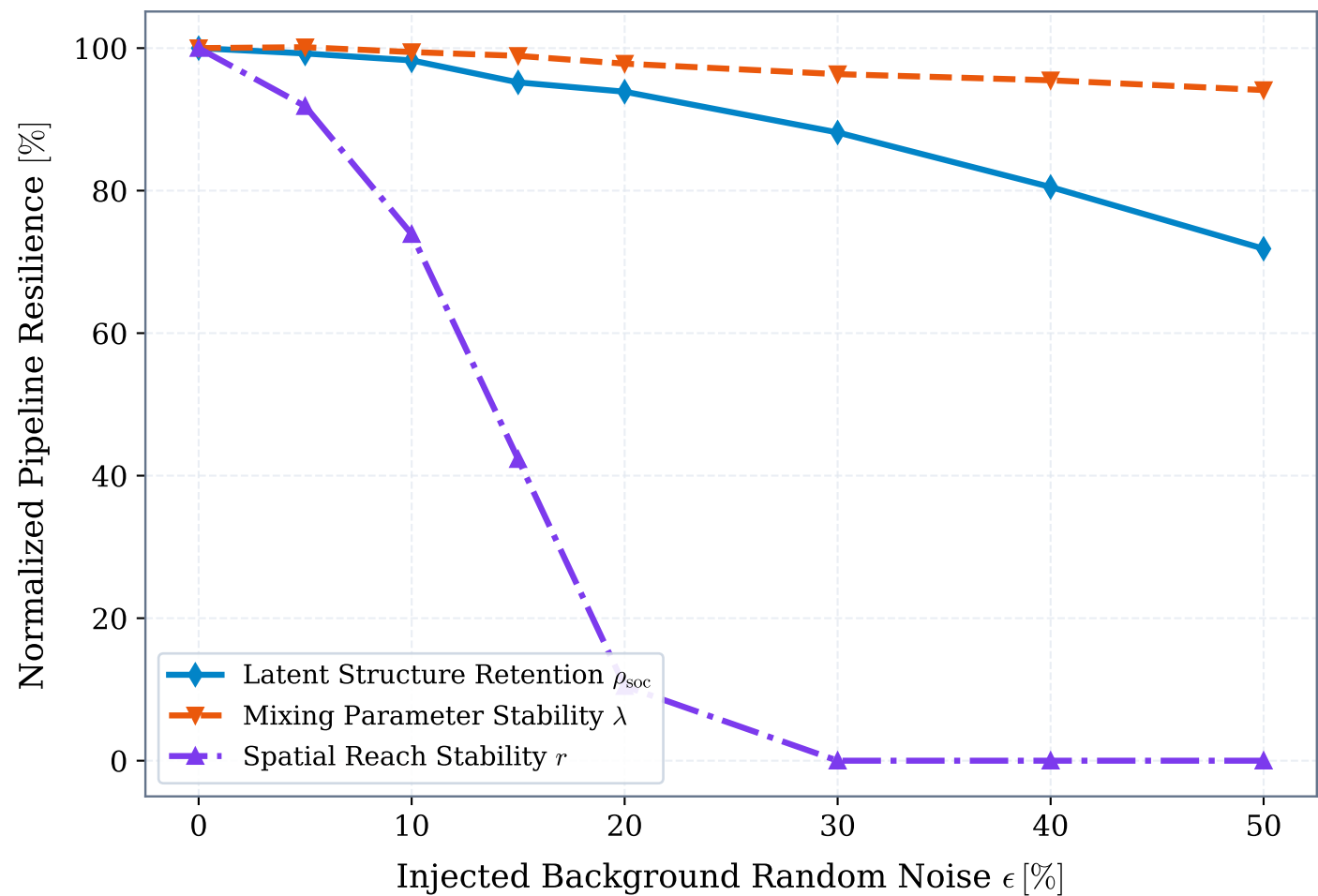
Normalized Pipeline Resilience under Noise
