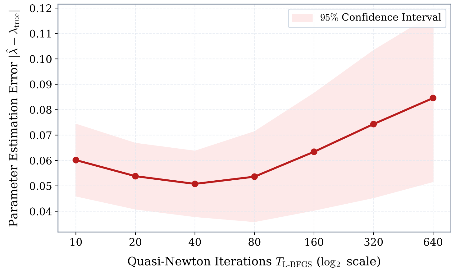
(a) Parameter Recovery Accuracy
