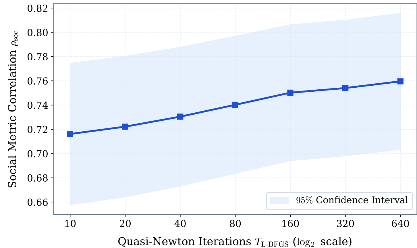
(b) Latent Metric Convergence
