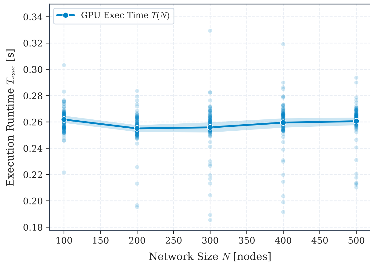
(a) Computational Weight \&amp; Wall-Clock Scaling
