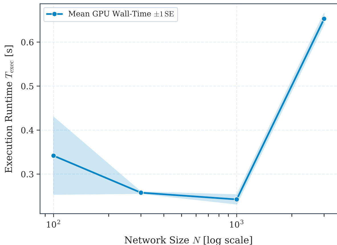
(a) Computational Runtime vs. \log N
