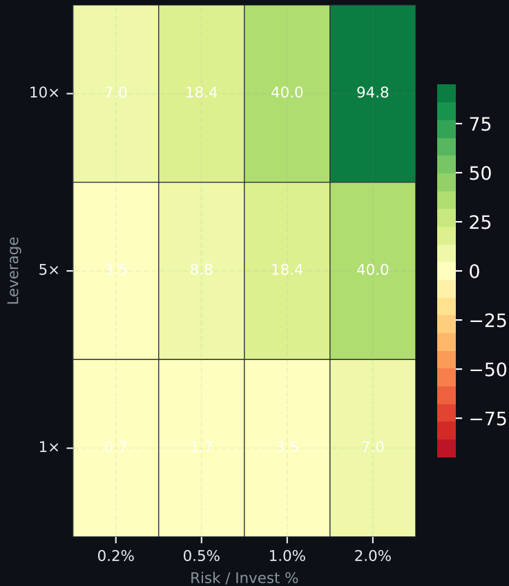
Fixed Fraction - Total Ret (%)
