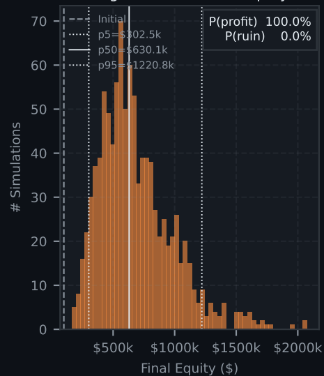
Regime filter – Final Equity
