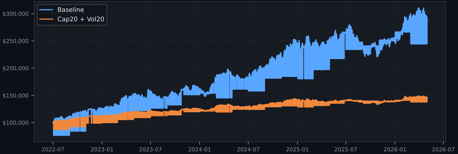
OOS Walk-Forward Equity
