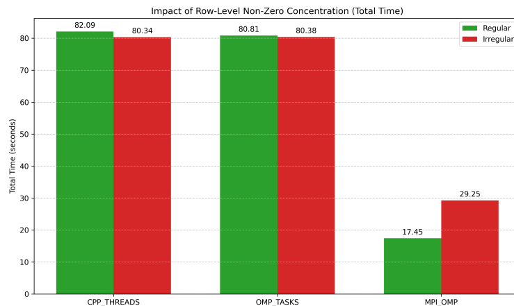
Figure 1: Impact of row-level non-zero concentration across implementations.
