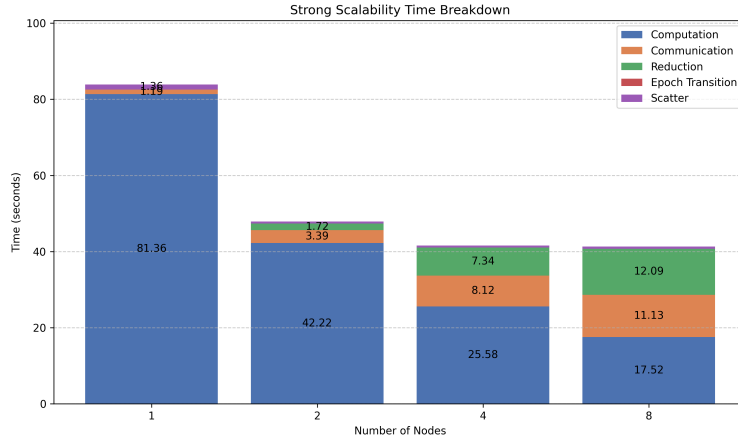
Figure 3: Per-rank peak time of each phase as the number of nodes increases.
