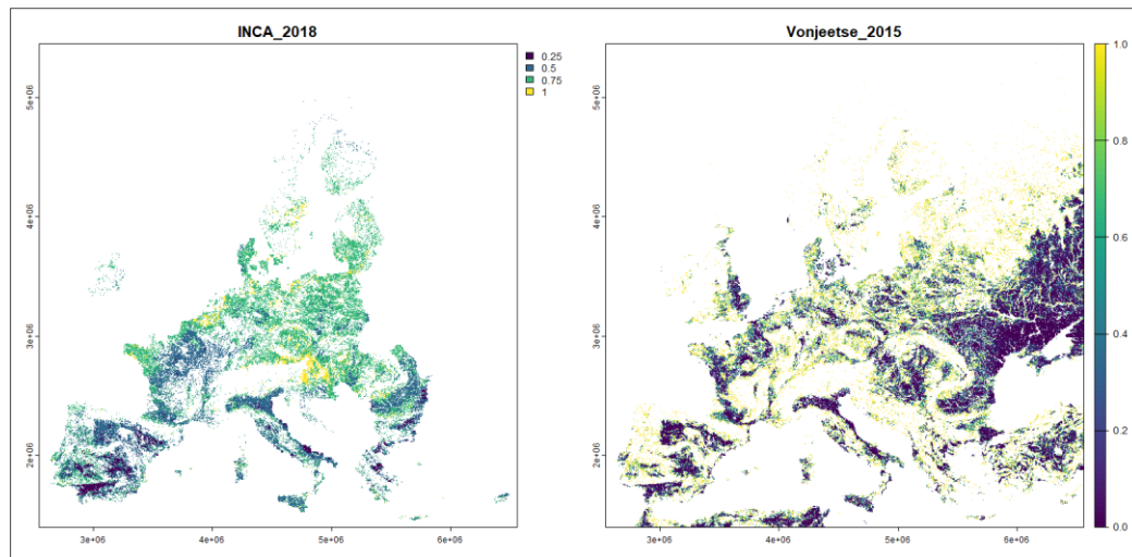
Comparison between von Jeetze et. al 2023 pollSuff_2015_Ref_10s and INCA_2018 pollination potential normalized to 0-1.
