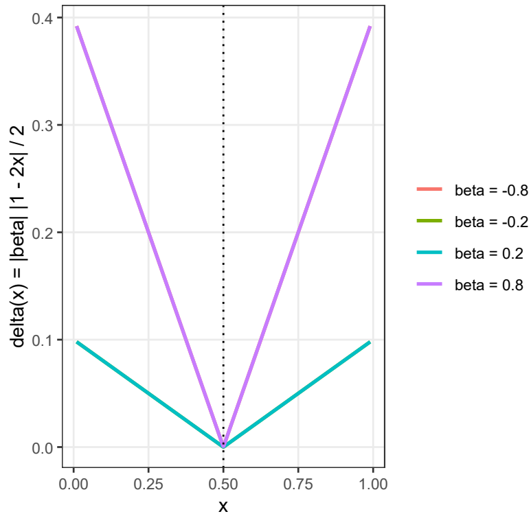
Copula-ratio sensitivity index
