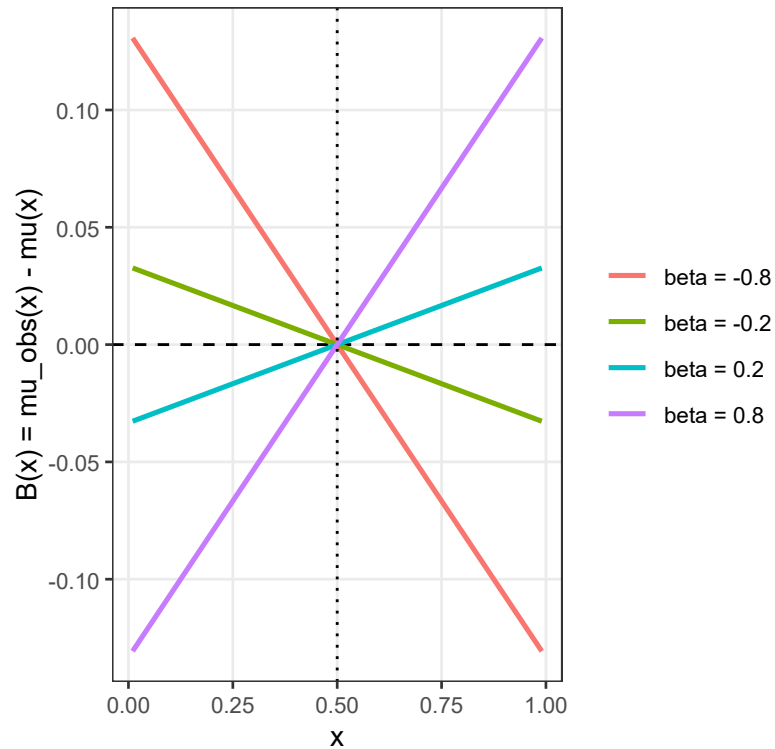
Confounding bias across treatment values
