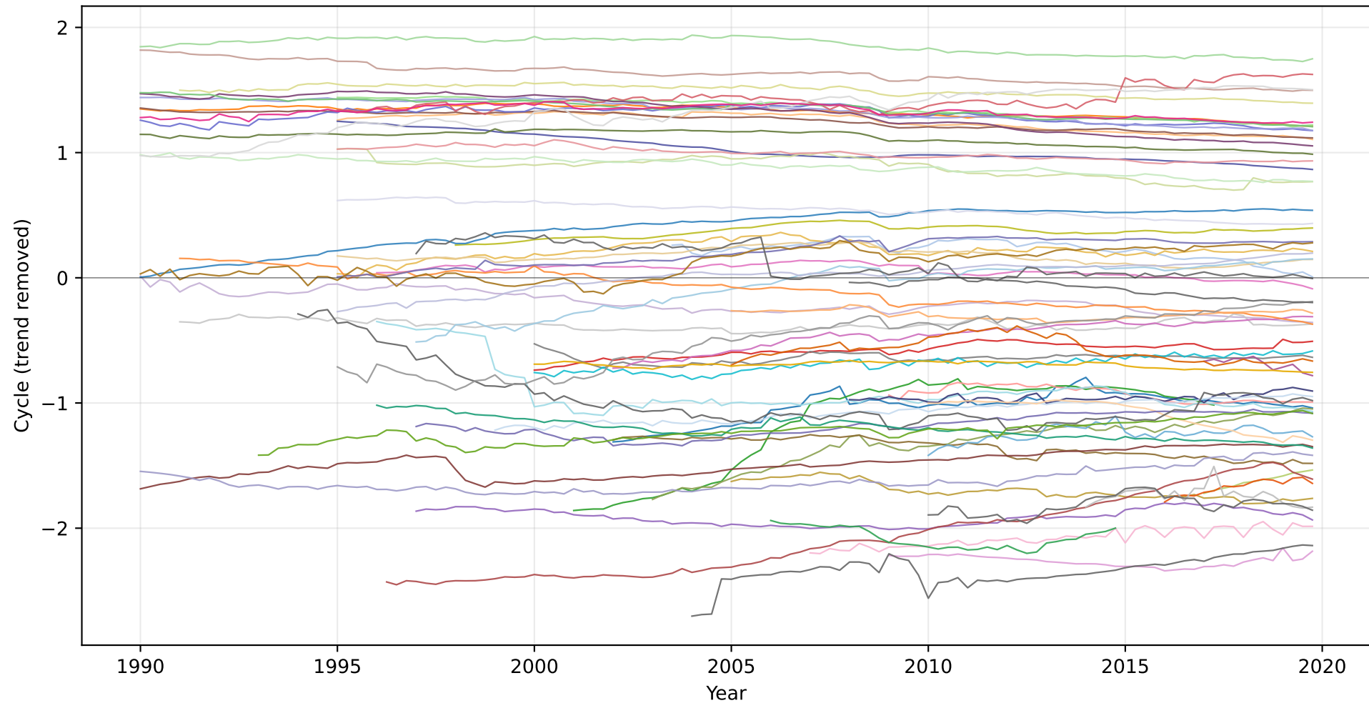
Common intercept and linear trend, 1990--2019, ex US, Germany, Japan, China
