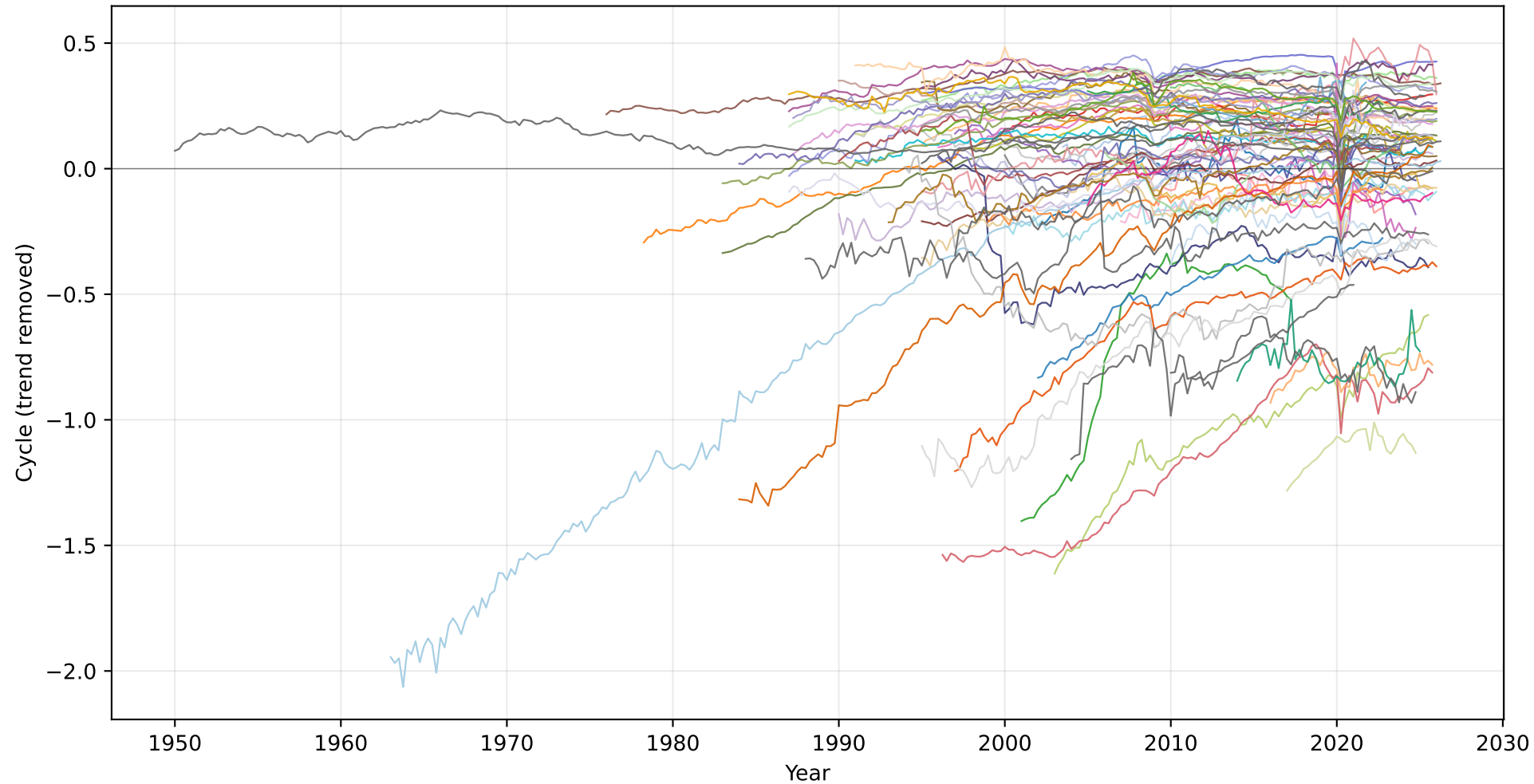
RE intercepts plus catch-up, lambda fixed at Barro 0.98
