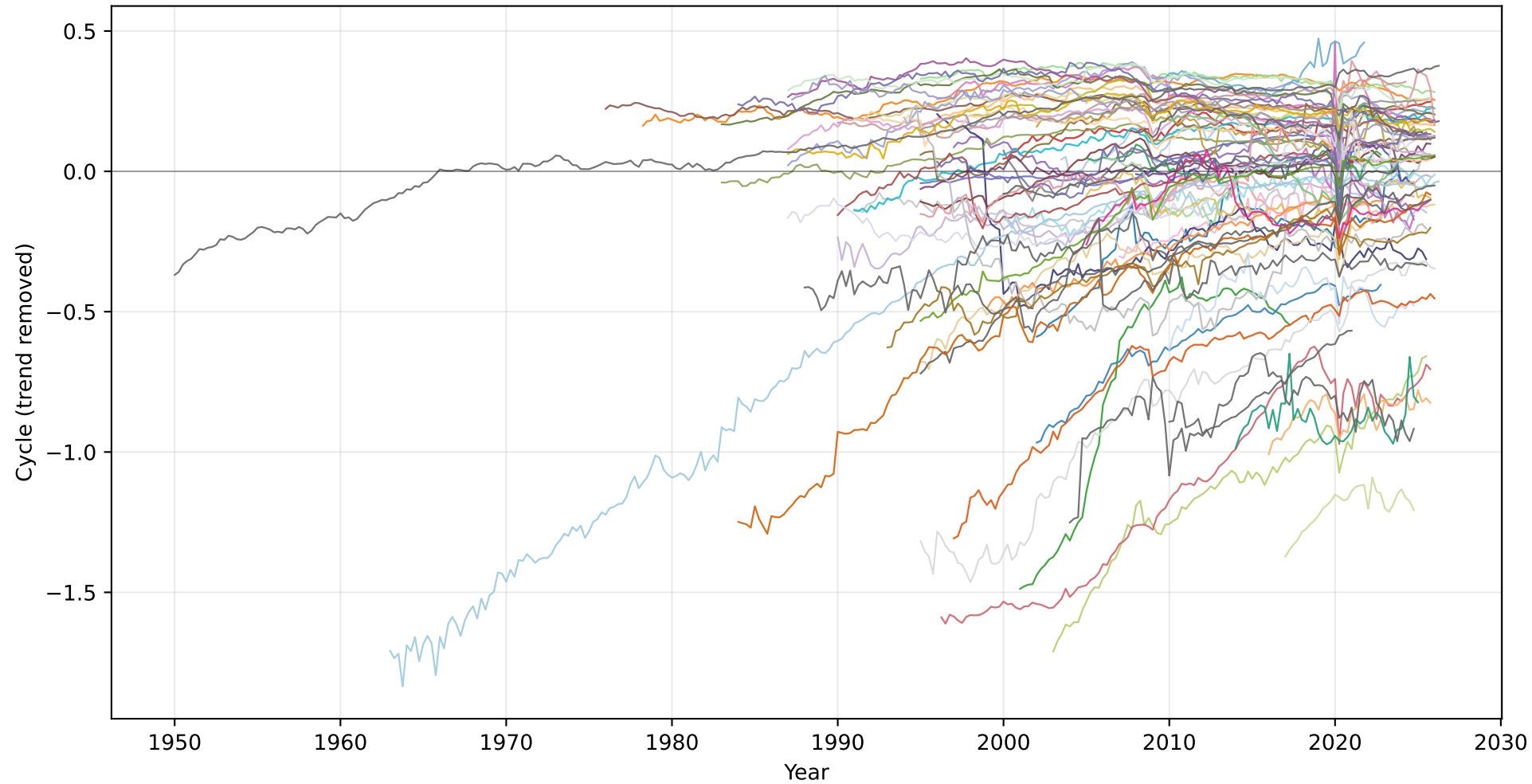
RE intercepts plus catch-up, free lambda in (0, 0.985)
