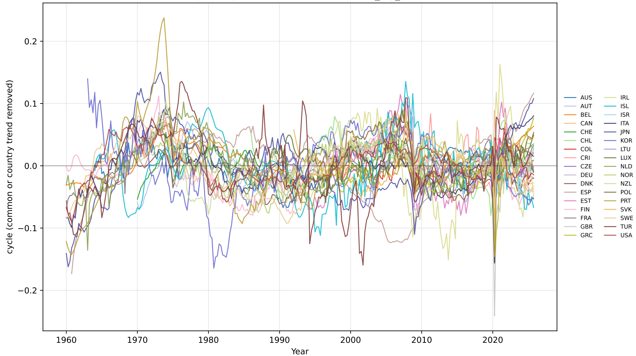
Two-step OLS quadratic-detrended series ( a_i , g_i , h t^2 )
