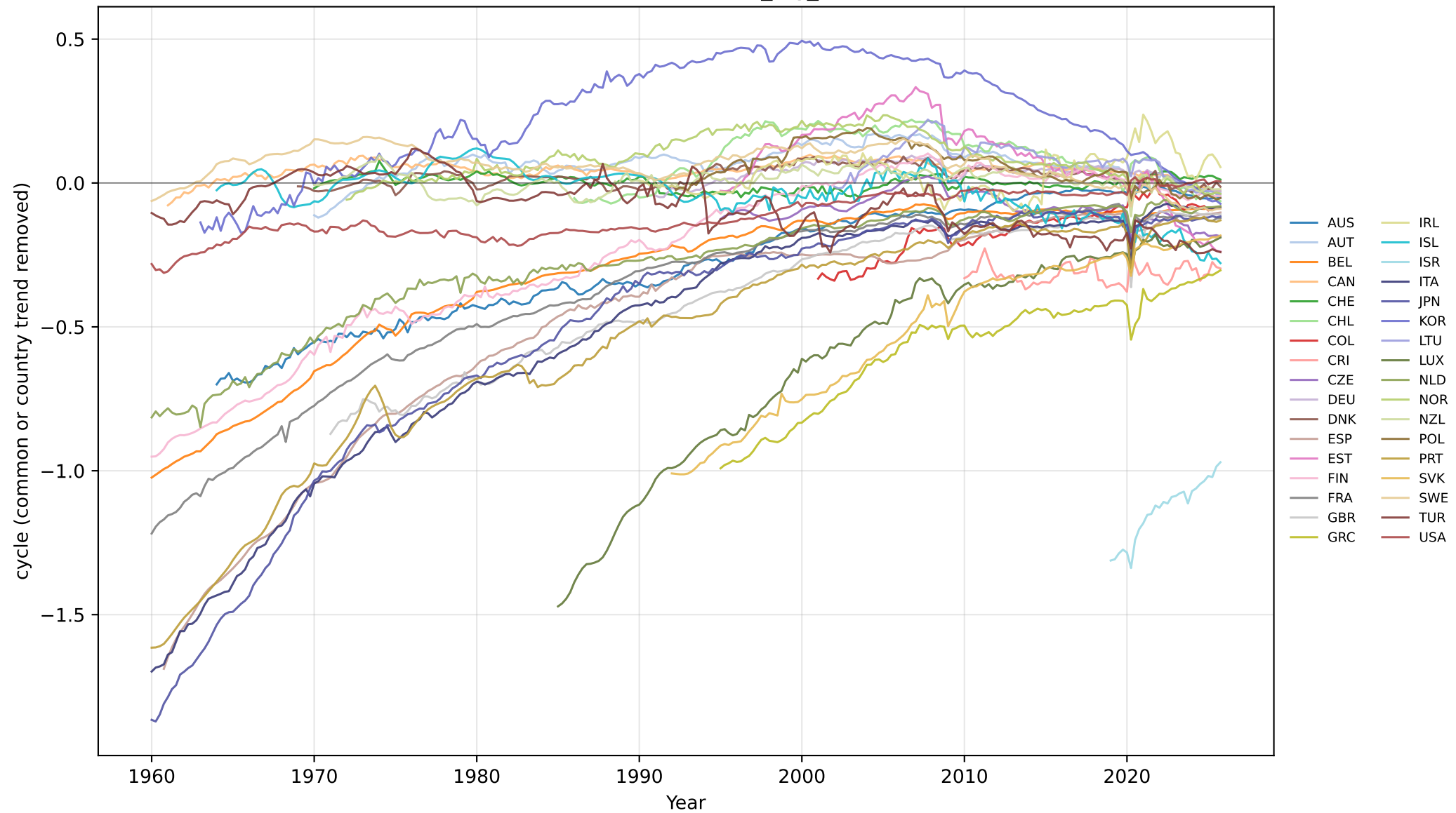
Detrended series (a_i, g_i)
