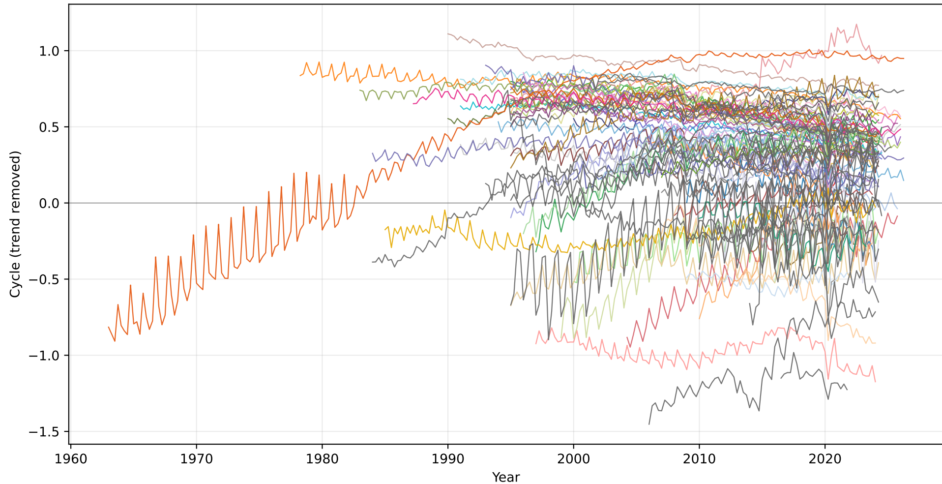
Pareto RE intercepts, common trend and quarterly dummies
