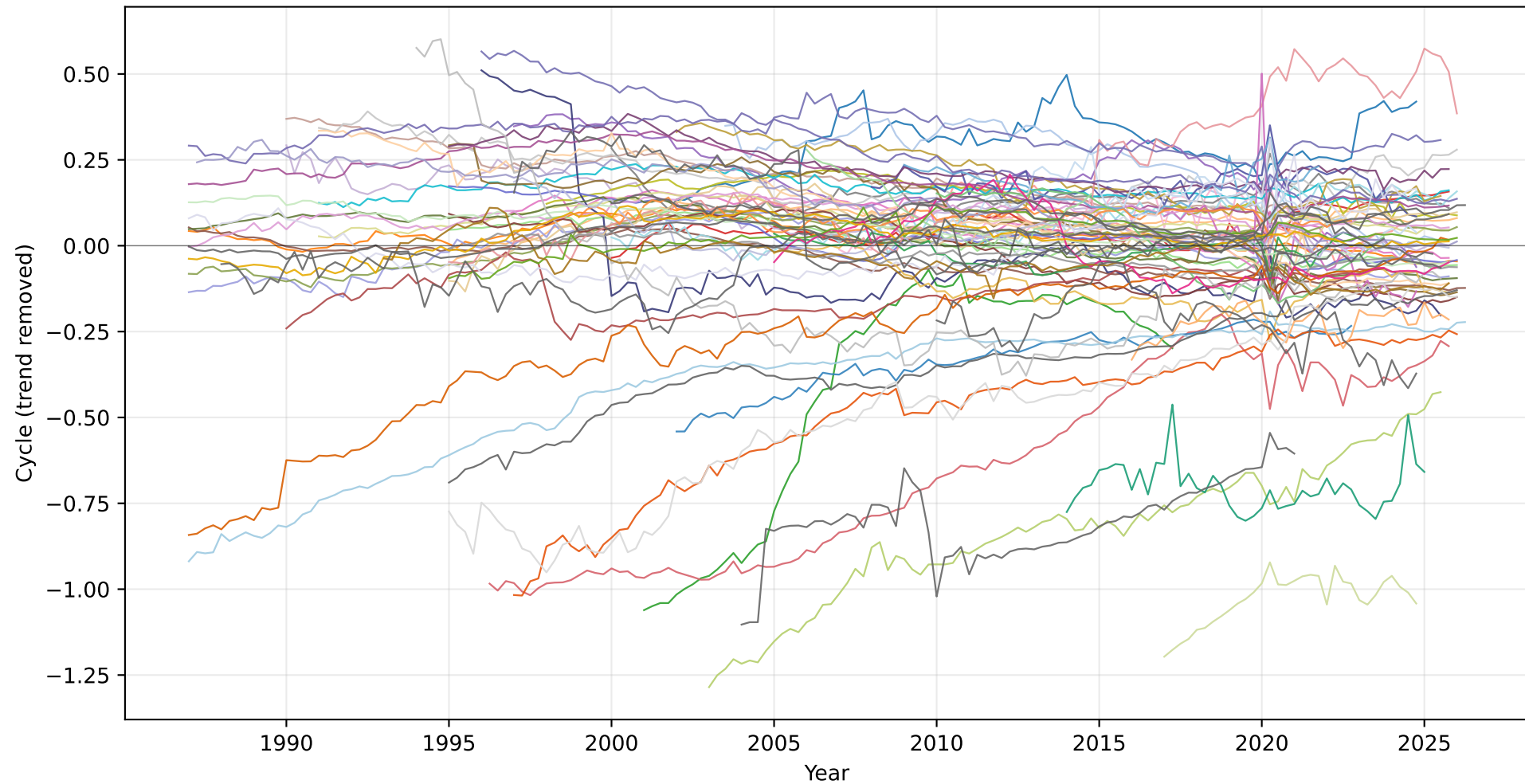
Common RW trend removed; RE intercepts plus catch-up, \lambda=0.99
