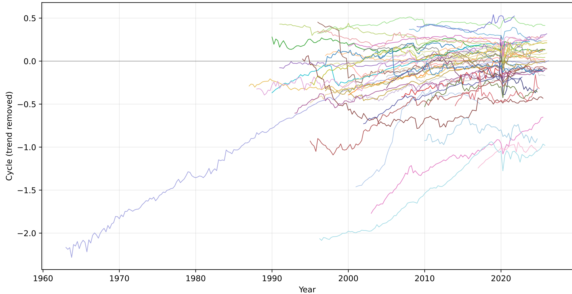
EMBI countries: random intercepts and a common linear trend
