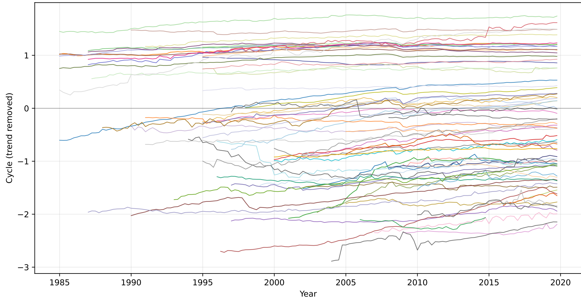
Common intercept and linear trend, 1985--2019, ex US, Germany, Japan, China
