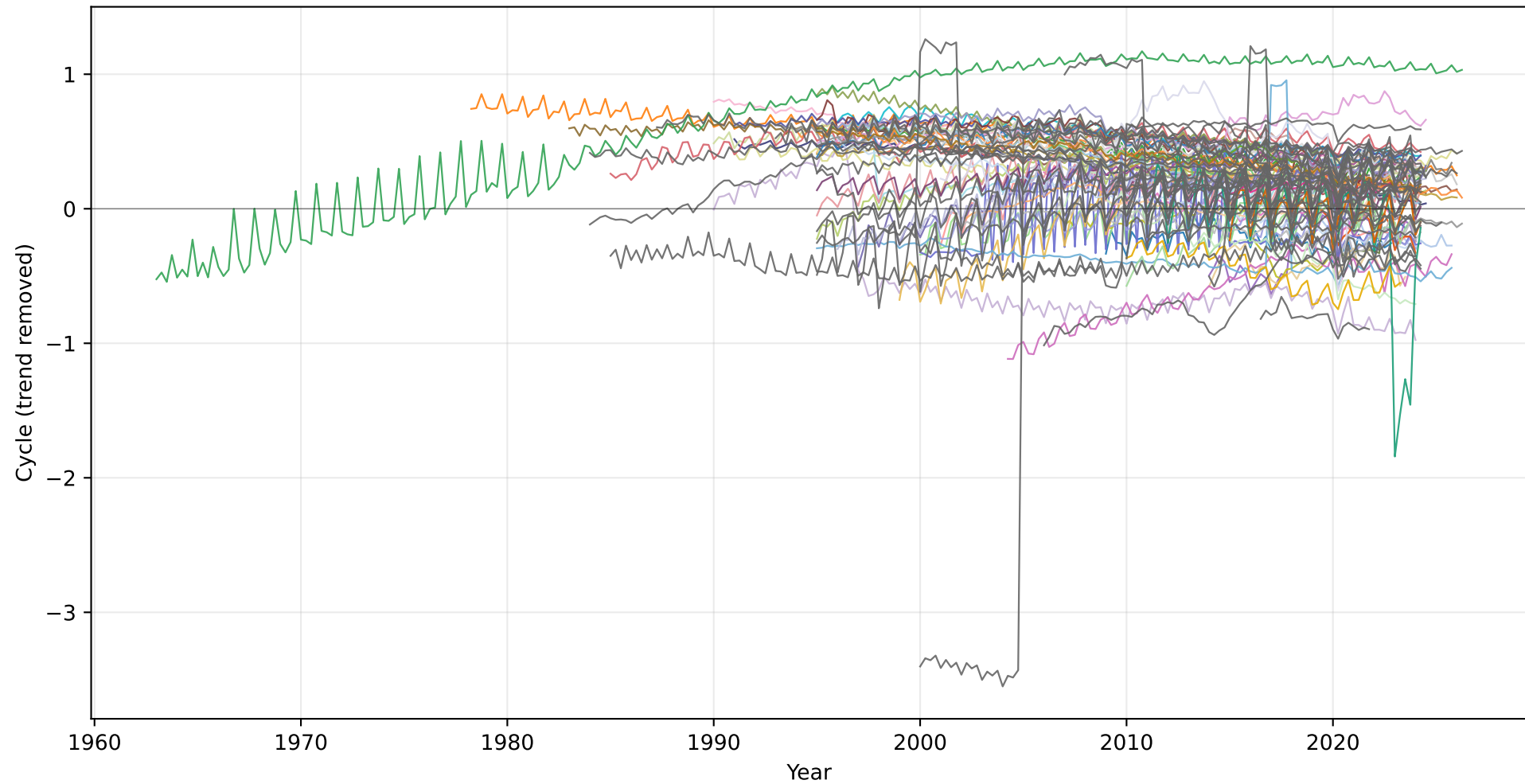
Random-effects intercepts, common linear trend
