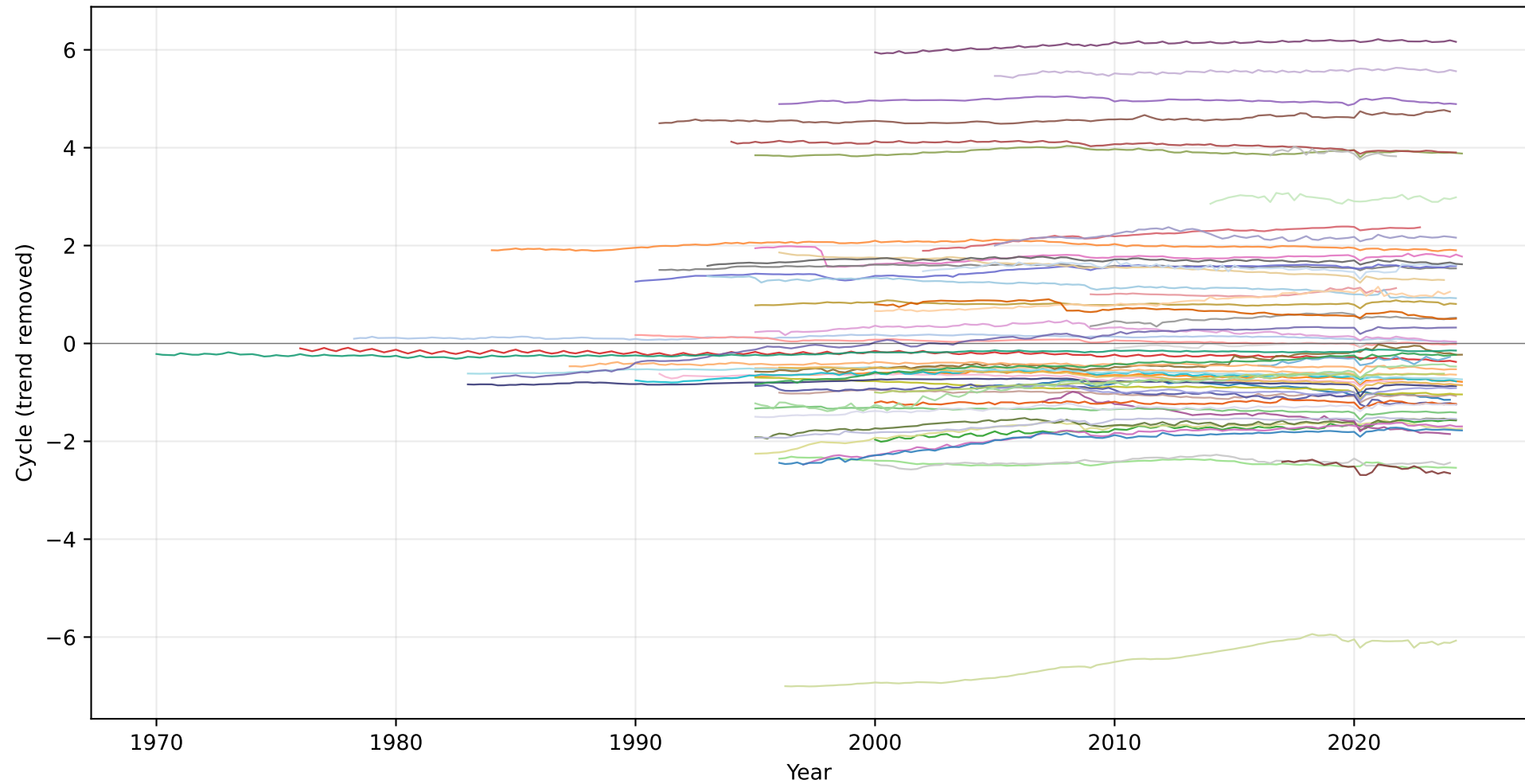
Common intercept and linear trend
