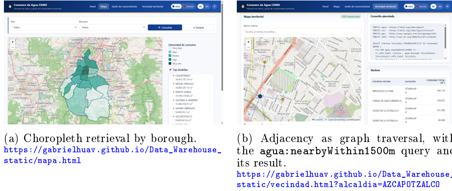
Fig. 1: The two retrieval modes of the static demonstration, both running in the browser without a server; each caption links to the exact view captured. Base map © OpenStreetMap contributors (ODbL).
