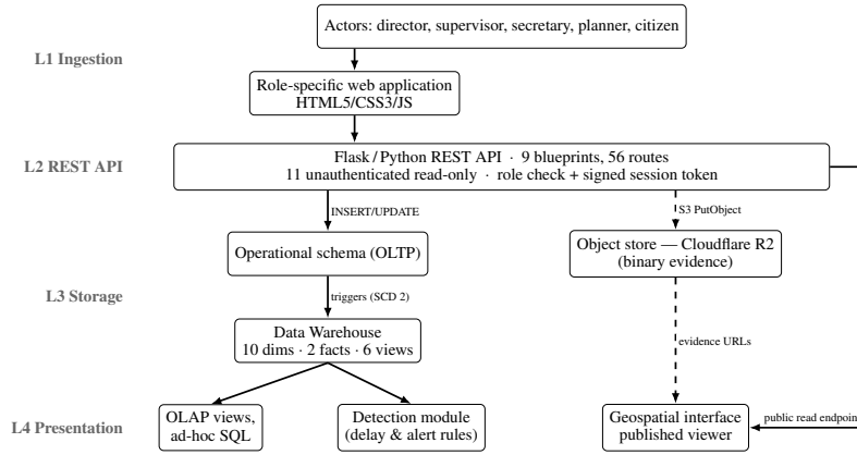
Fig. 1. System architecture (warehouse-centric): the analytical core is the dimensional Data Warehouse and the object store (labeled “Data Lake”) , redrawn in the figure) acts as the evidence layer. The four layers L1–L4 correspond to Sections 3.1–3.4. Solid arrows: structured-data flow; dashed arrows: unstructured-data unstructured (binary) evidence flow. Released role-specific pages read operational endpoints; the warehouse serves detection and OLAP through /api/analitica . The geospatial viewer is part of the released artefact.
