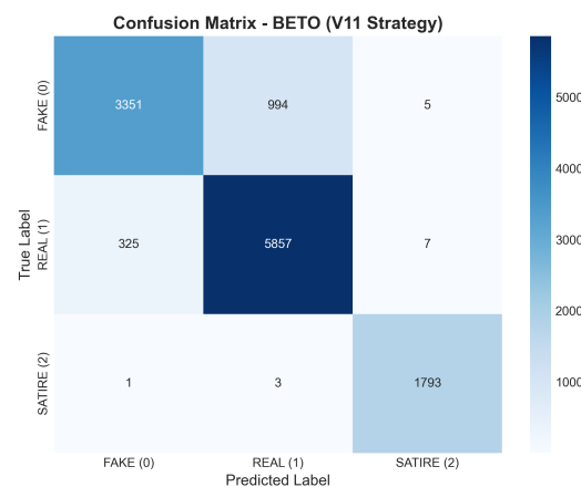
Figure 8. Confusion matrix of the final three-class BETO model (the deployed model) on the held-out test set, distinguishing Fake (Class 0), Real (Class 1), and Satire (Class 2). This is the confusion matrix corresponding to the main results of the paper, in contrast to the preliminary binary matrices in Figure 6.
