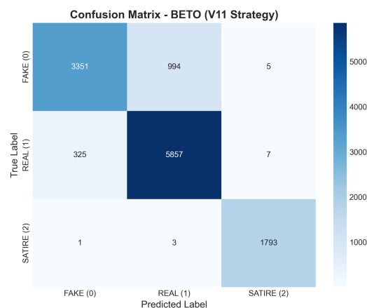
Figure 8. Confusion matrix of the final deployed BETO model on the held-out test set, showcasing its robust capacity to differentiate between Fake (Class 0), Real (Class 1), and Satirical (Class 2) content.
