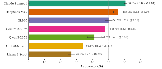
Figure 3: GeoNatureAgent Benchmark v5 leaderboard. Accuracy (%) with total cost in parentheses. Dashed line at 50%.
