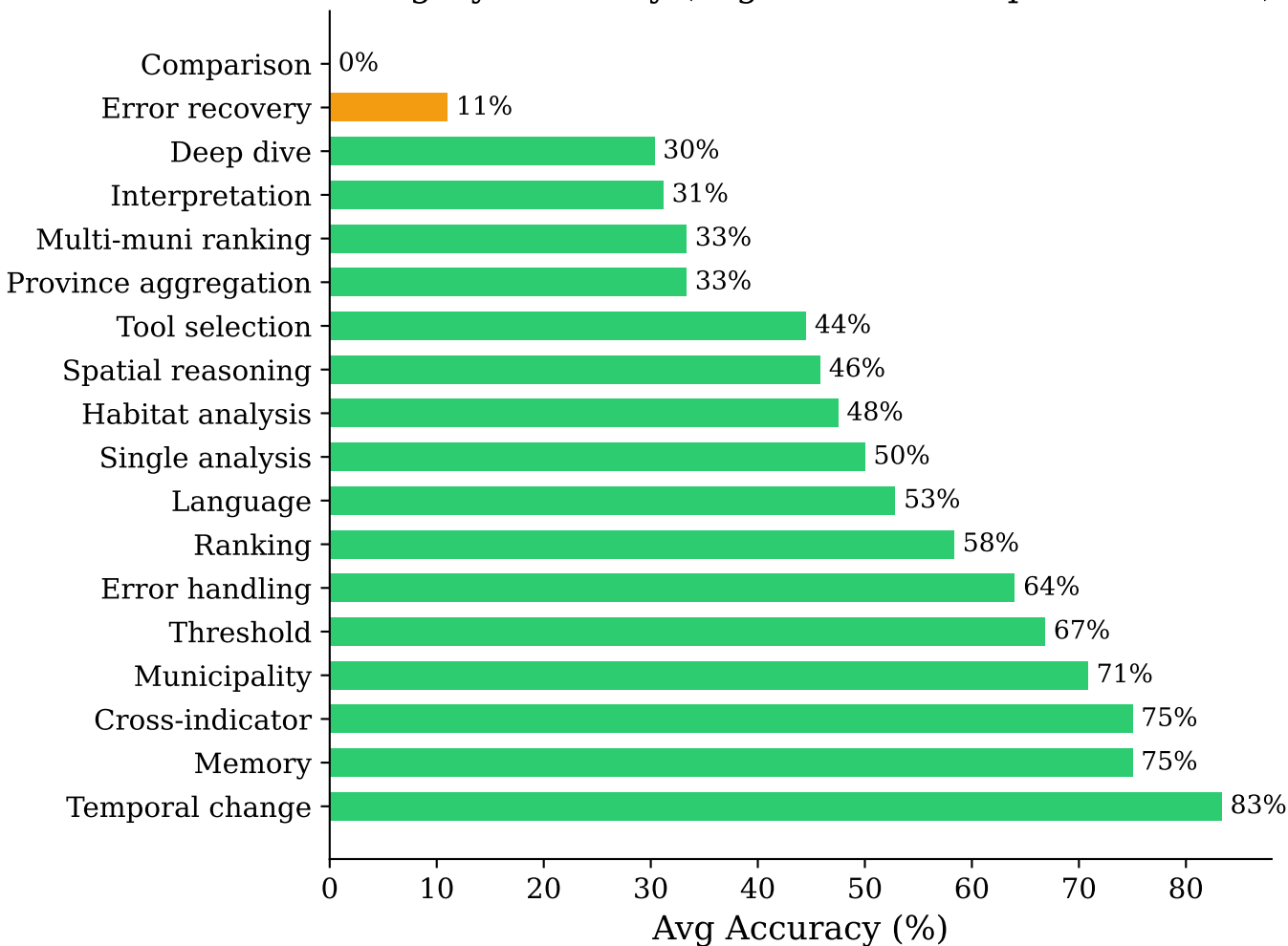
Category Difficulty (avg across 6 completed models)
